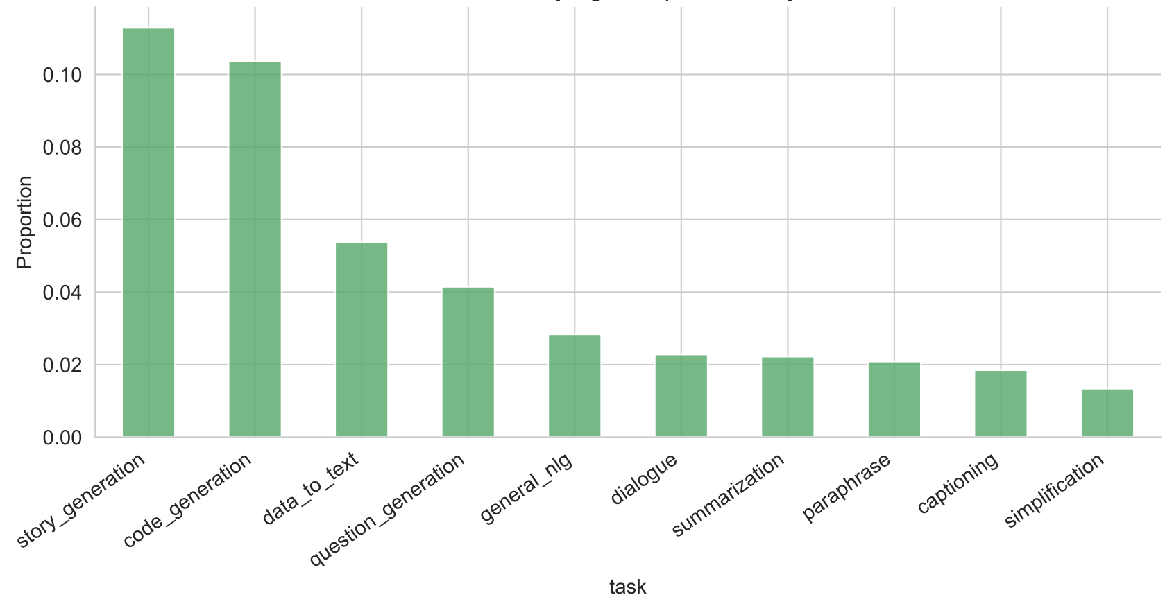
RQ2: LLM-as-judge adoption rate by task
