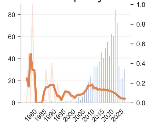
adequacy
