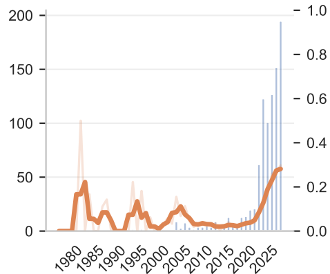
faithfulness
