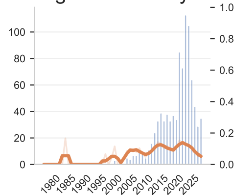
grammaticality
