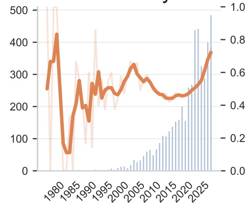
accuracy
