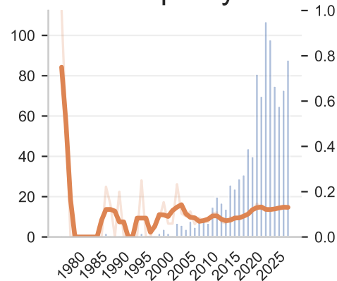
simplicity
