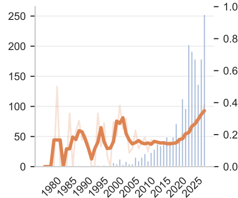
relevance
