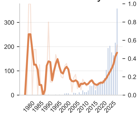
consistency
