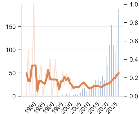
correctness
