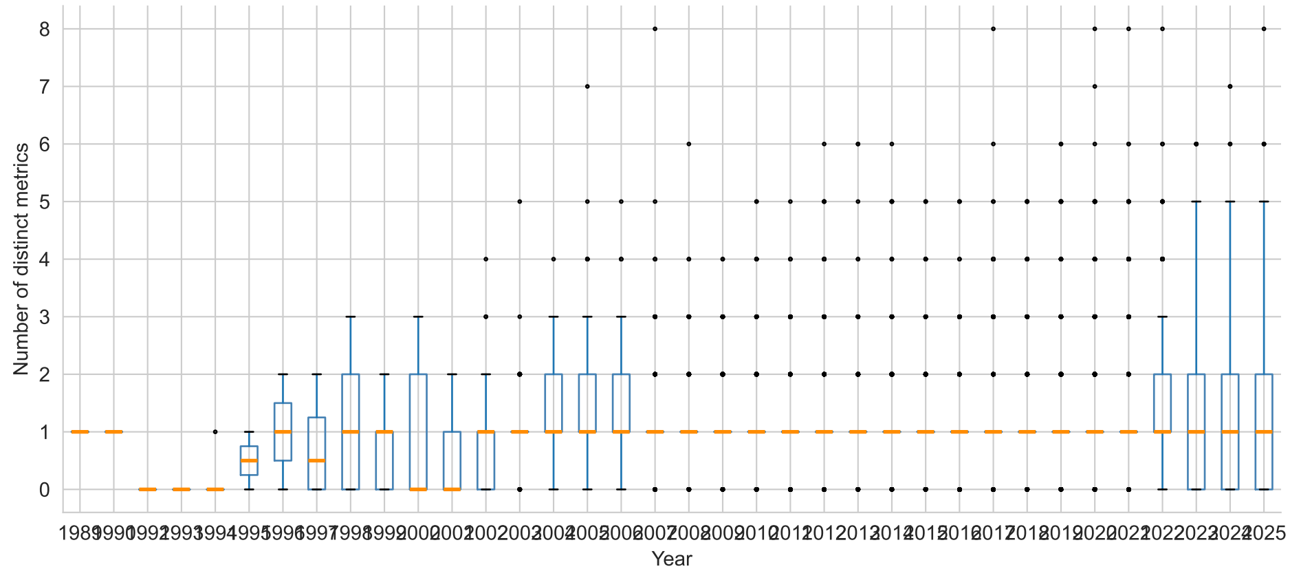
RQ5: Metric diversity per paper by year
