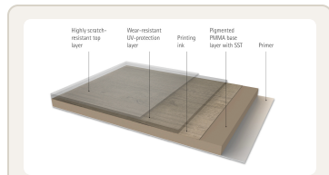
FIGURE 1. TRUEGRAIN LAMINATE CROSS-SECTION. LAYERS SHOWN IN TRUE STACKING ORDER, TOP TO BOTTOM.
