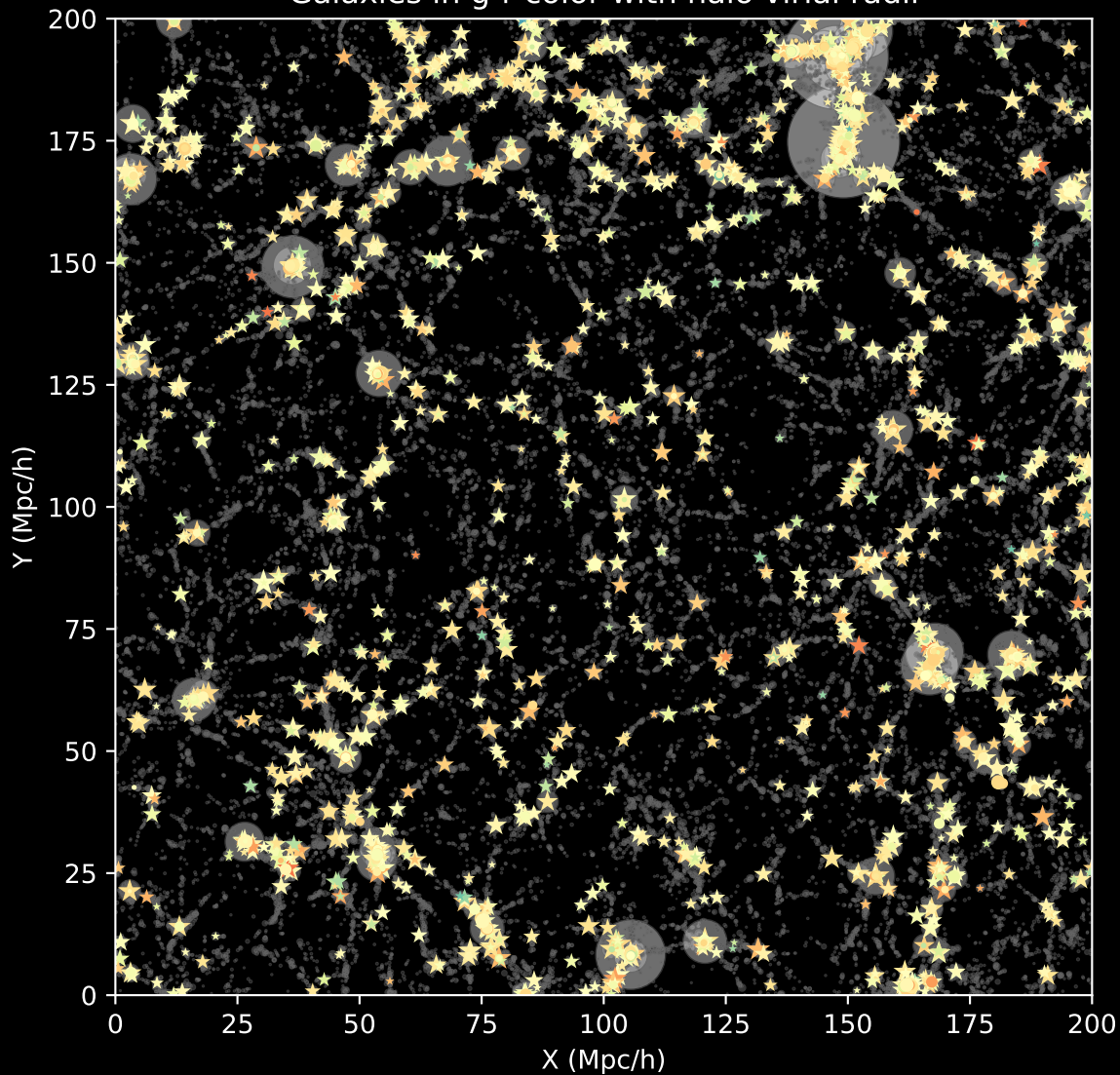
Galaxies in g-r color with halo virial radii
