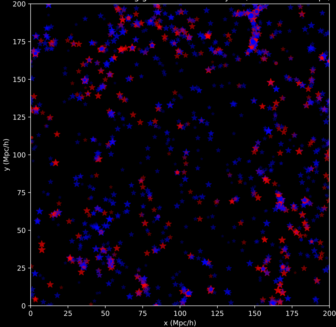
Galaxies of the BGS catalog generated from Sahyadri, slice Z=100.0 Mpc/h
