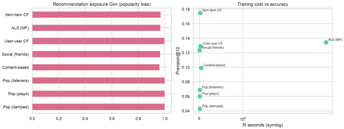
Figure 6. Popularity bias via exposure Gini (left) and training cost versus accuracy (right).
