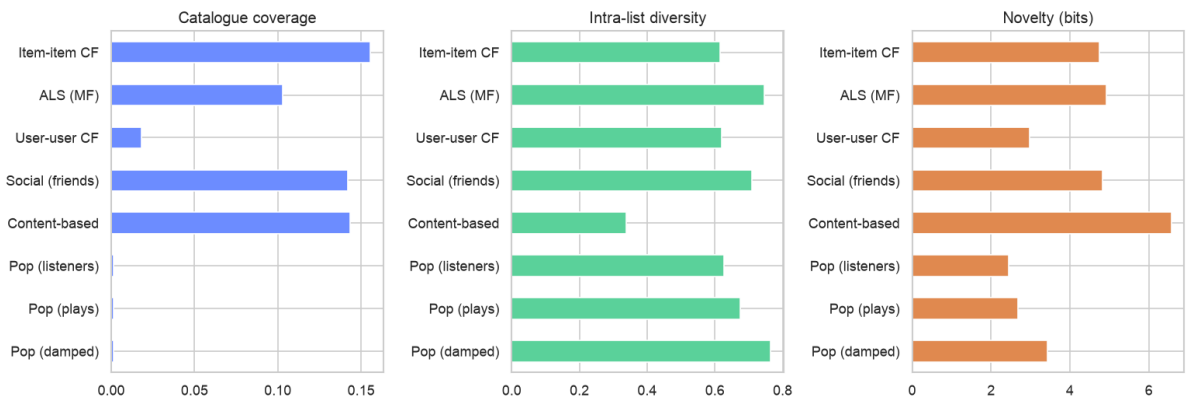
Figure 4. Beyond-accuracy metrics: coverage, diversity, novelty.
