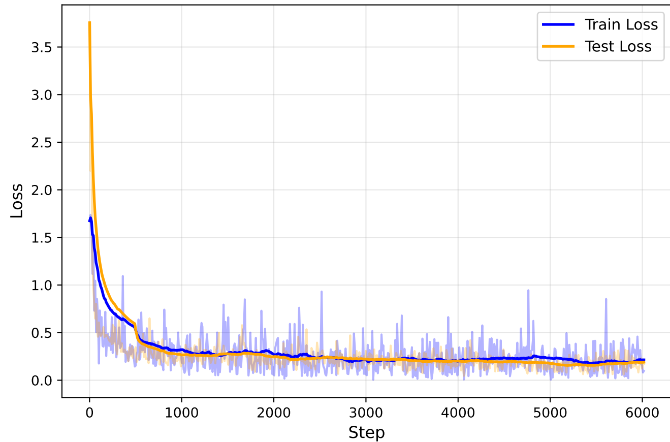
Multiclass CNN - Loss
