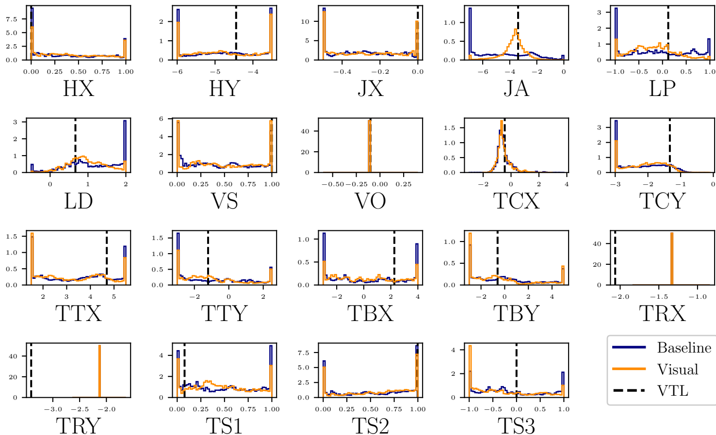
Distributions of articulatory states corresponding to phoneme category: /R(a)/
