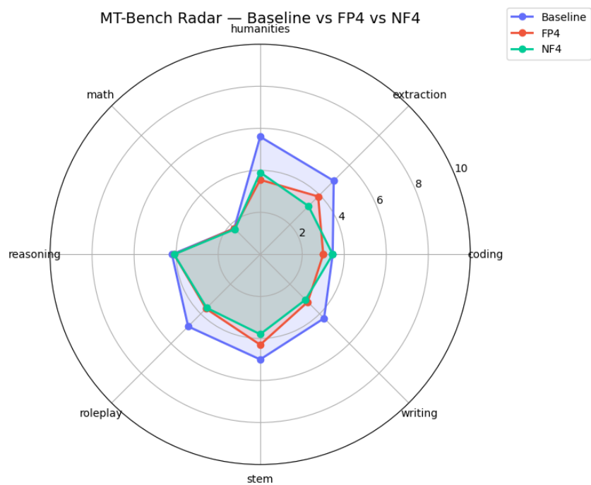
Figure 4: MT-Bench Radar Chart — Baseline vs. FP4 vs. NF4. Radar visualization of per-category scores. The Baseline (blue) occupies a noticeably larger area, particularly in the humanities and STEM, while FP4 and NF4 (orange and green) overlap closely, suggesting similar quantization-induced degradation patterns across both formats.
