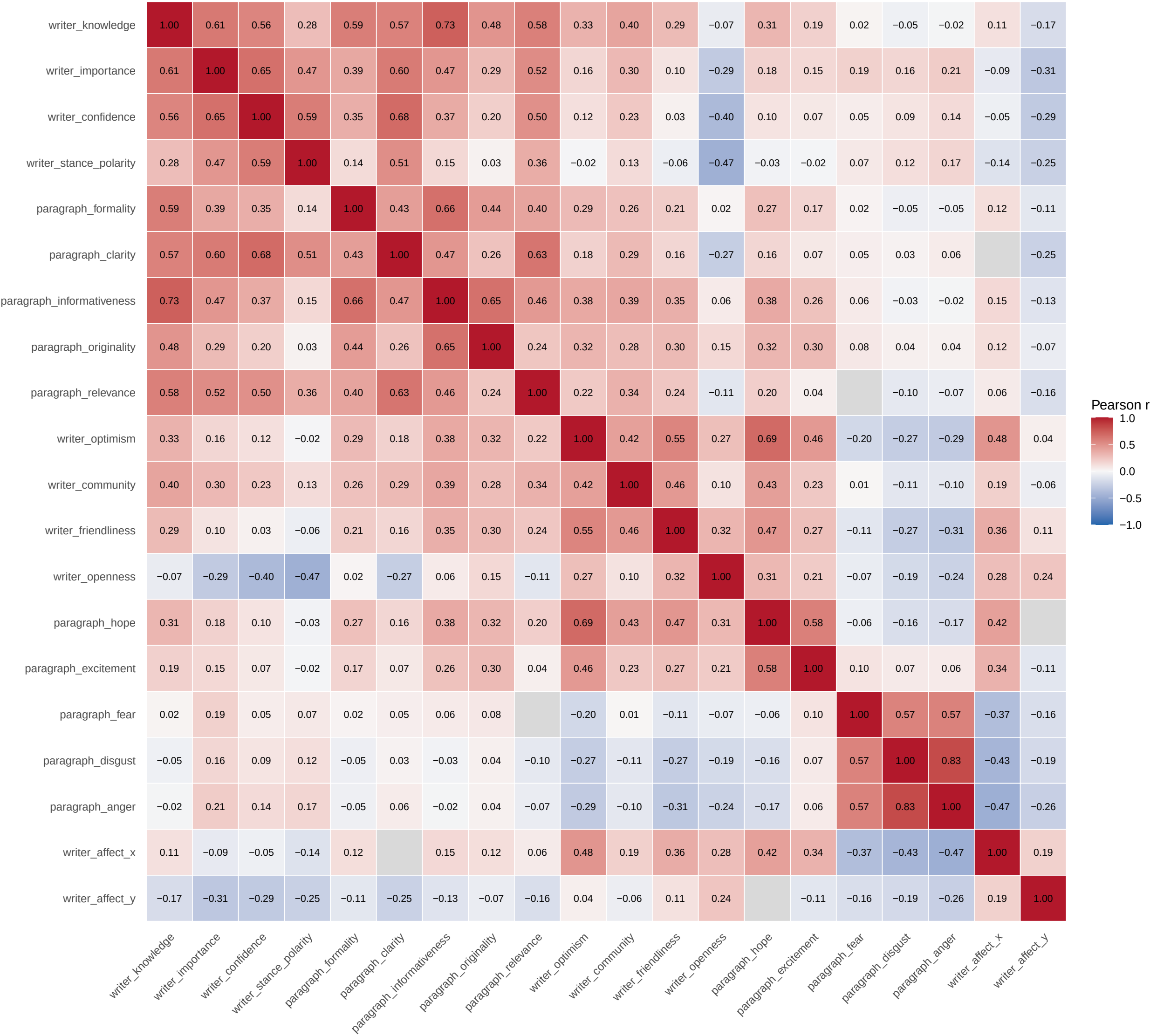
Scale Attribute Correlations: Edited
