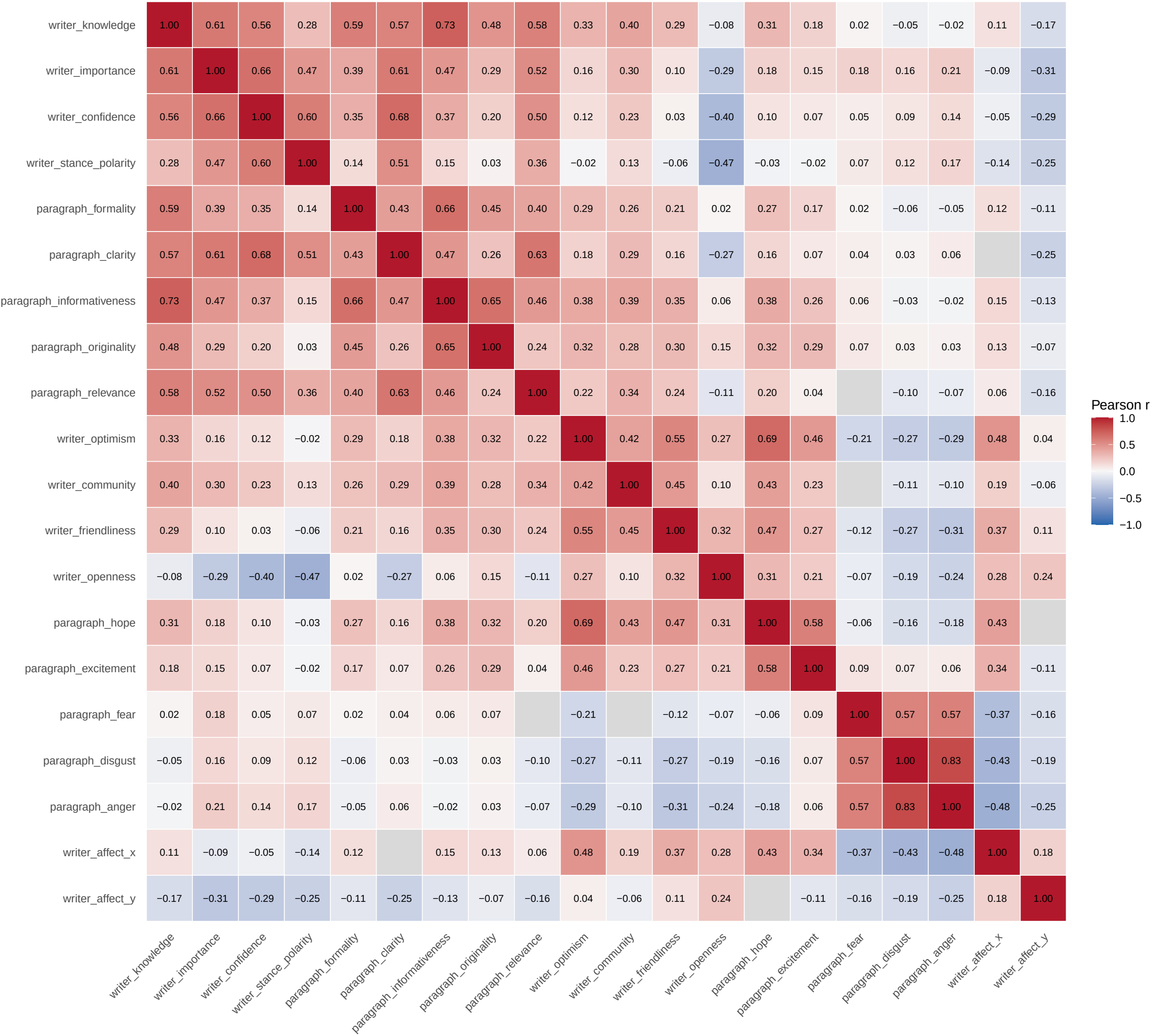
Scale Attribute Correlations: Unedited
