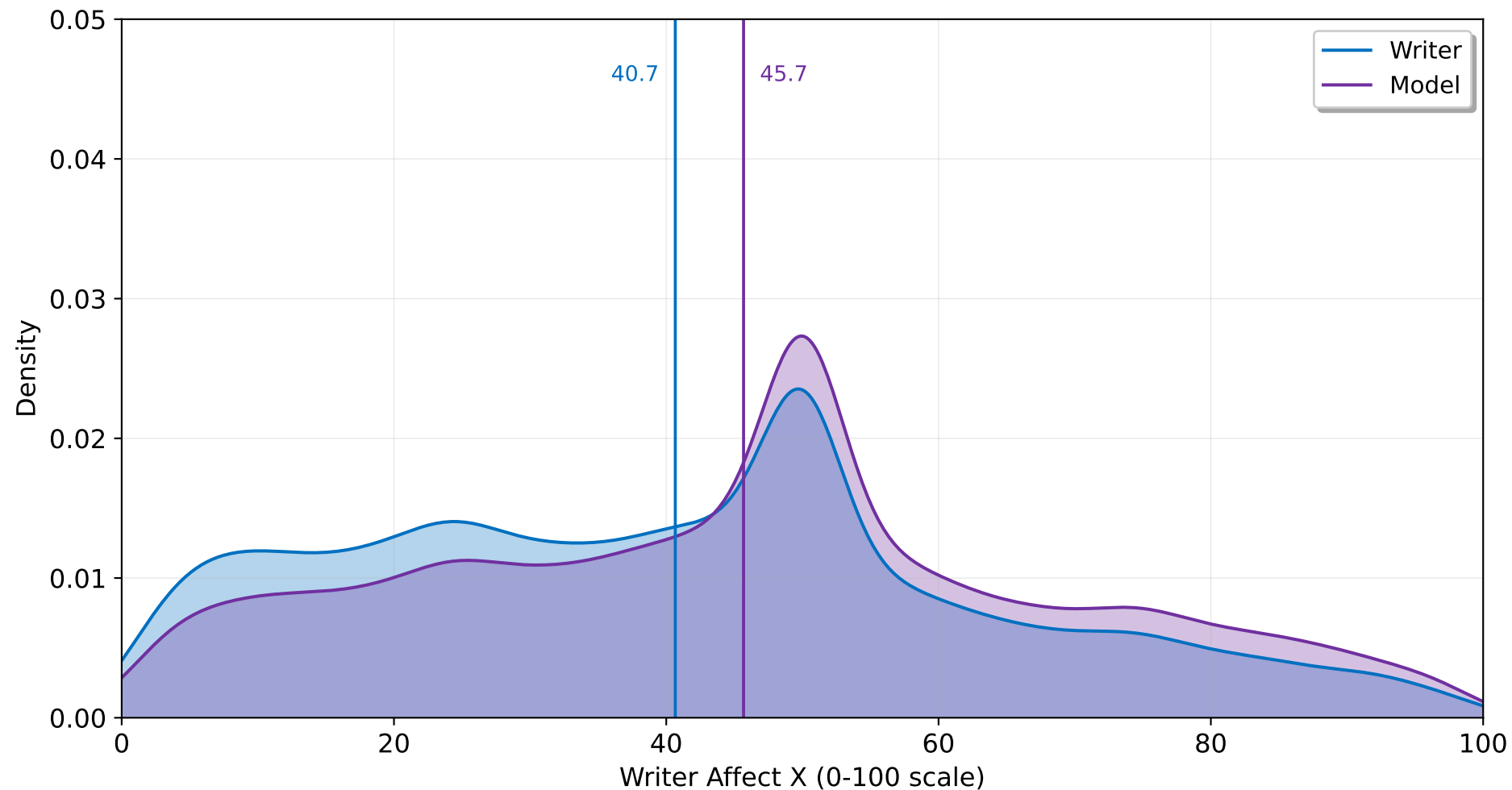
Distribution of Writer Affect X Ratings Writer vs AI Model Generated Paragraphs
