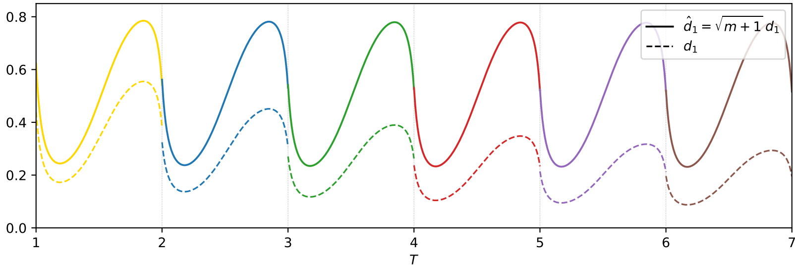
d_1 and \hat{d}_1 on the critical line, 1 < T < 7
