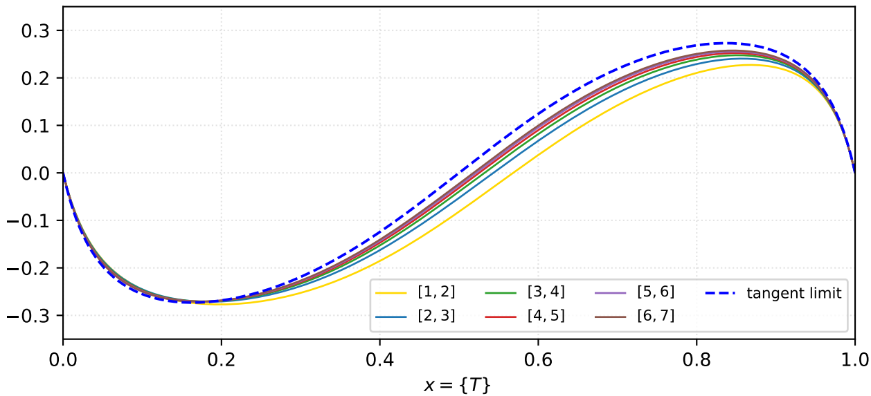
\mathcal{W}(T) overlaid, against the tangent limit
