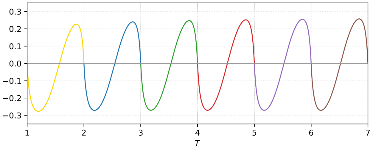
\mathcal{W}(T) continuous and periodic
