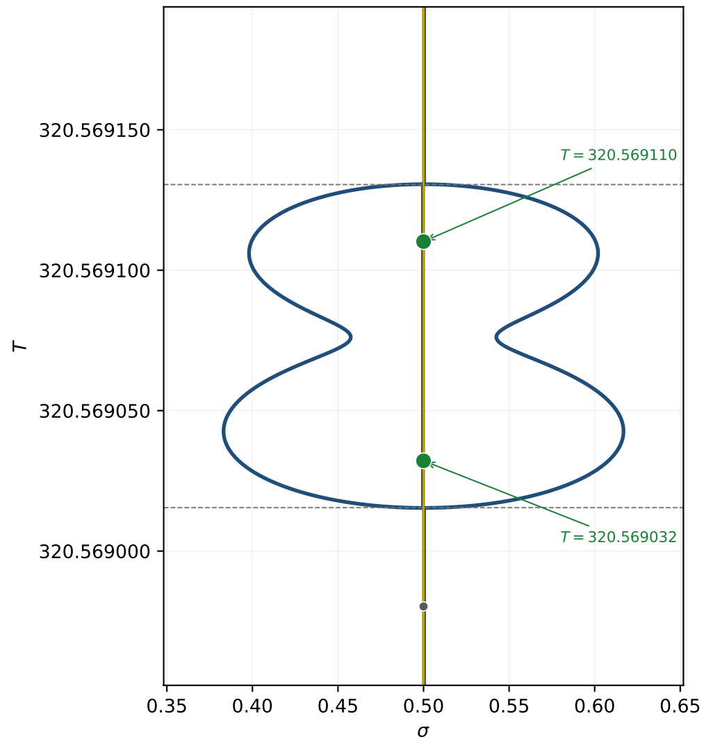
AK oval holding two zeros, T \approx 320.57
