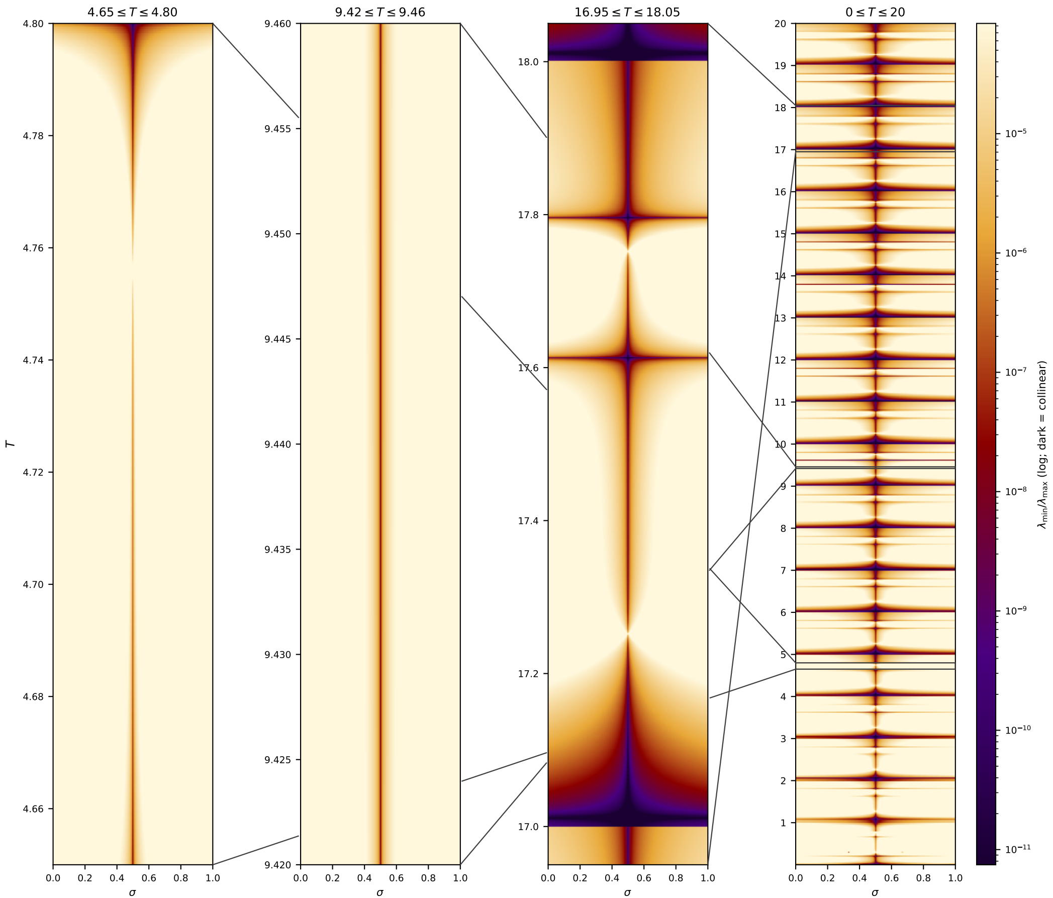
PCA aspect ratio \lambda_{\min}/\lambda_{\max} of (R_{1ps}, R_{1rs}, R_{1ak}) (dark purple = collinear) first three panels are zooms of the outlined bands on the right
