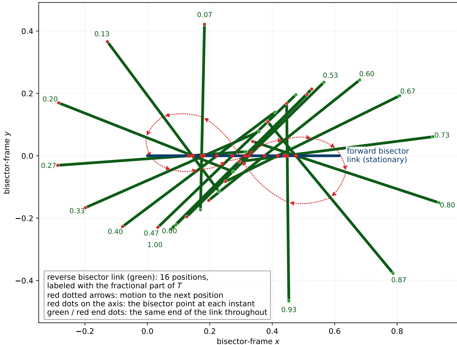
The reverse bisector link revolving around the forward bisector link: \sigma = 1/4 , T = 6 \rightarrow 7 , sixteen positions
