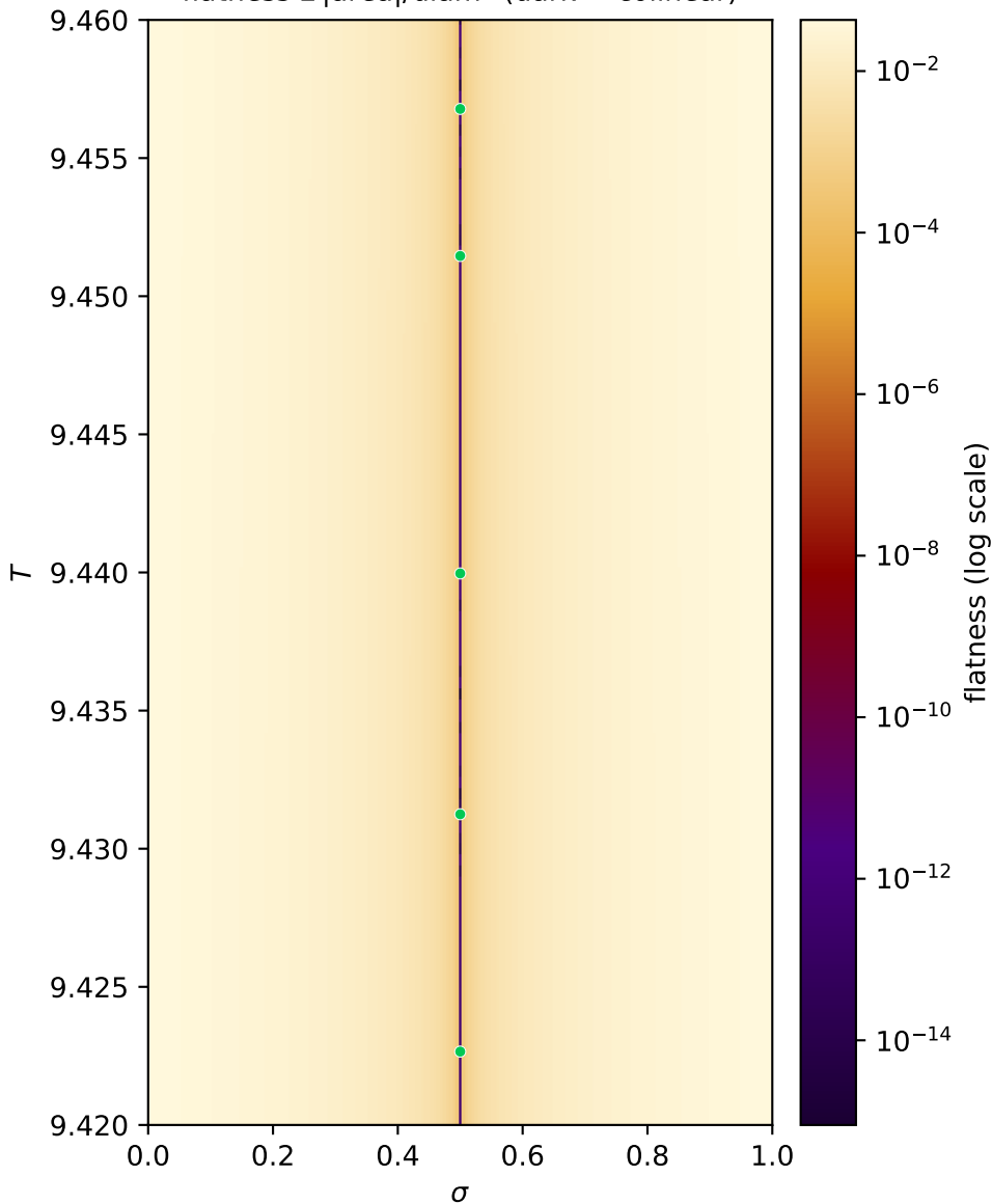
Colinearity of R_{1ps} , R_{1rs} , R_{1ak} flatness 2 |area|/diam 2 (dark = colinear)
