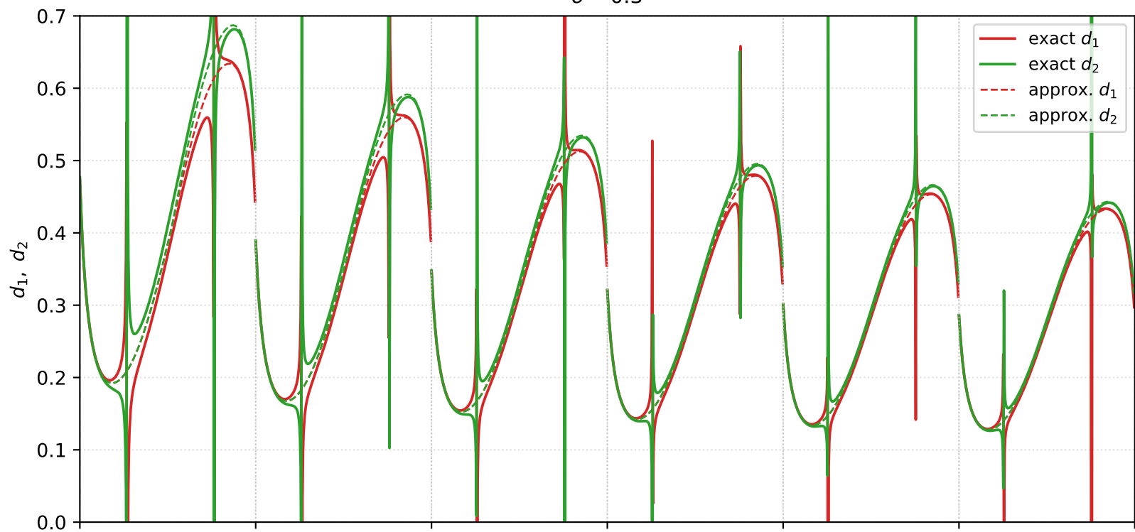
d_1 and d_2 across the strip: first-term approximation (no zeta input)
