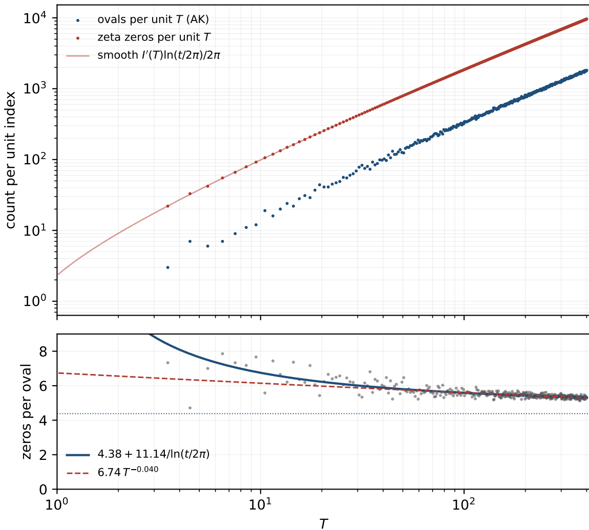
Equal-leg ovals and zeros per unit index, 1 \leq T \leq 401 , \sigma = 1/2 + 0.01
