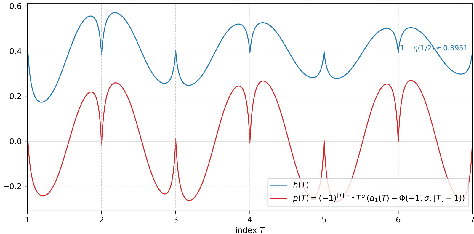
exactly continuous coordinates of the point B_1 ( \sigma = 1/2 ): flattening h vs. non-flattening p
