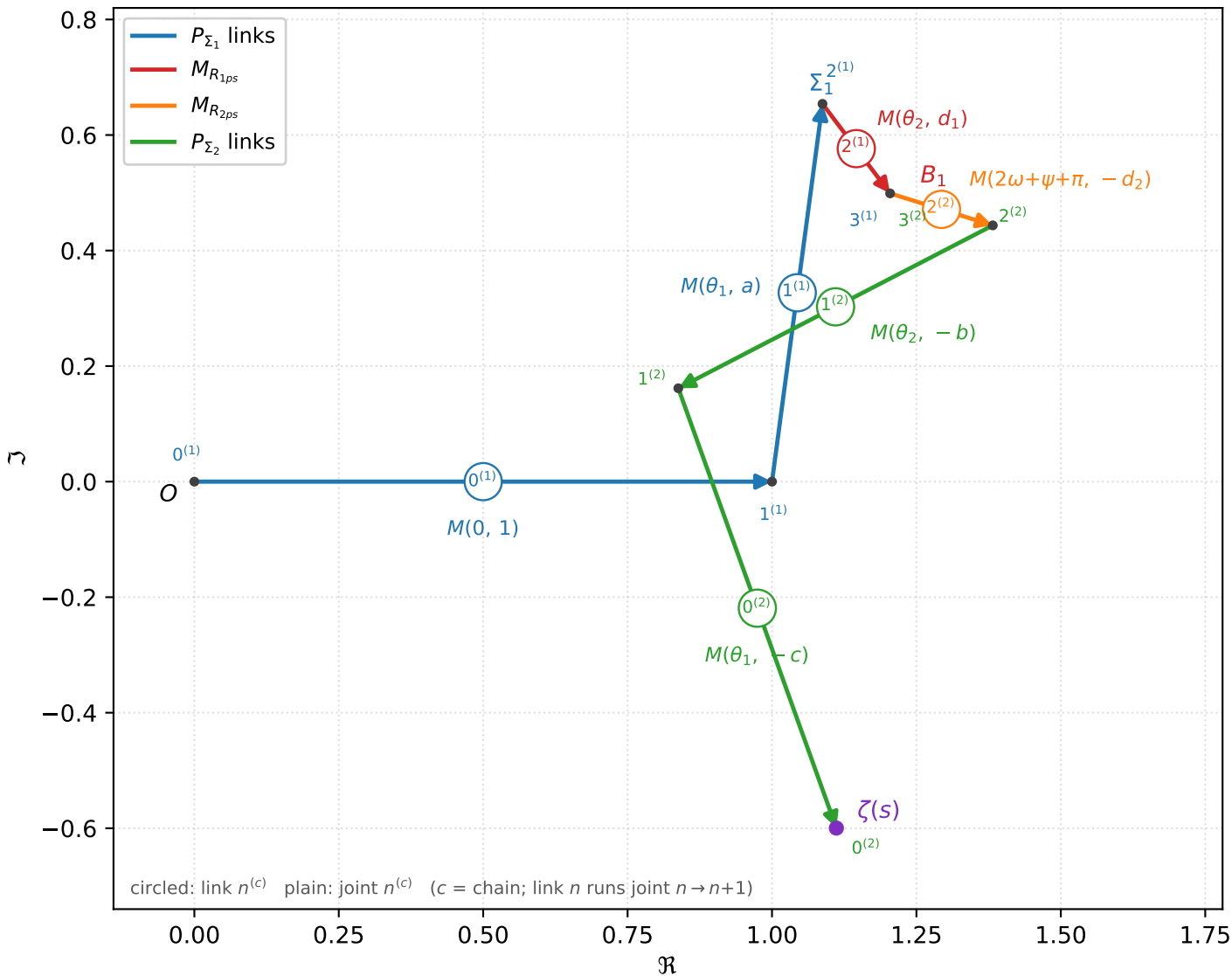
The six matrices of the m = 2 chain \sigma = 0.6 , T = 2.4 ( t = l(T) \approx 52.314 ), m = 2
