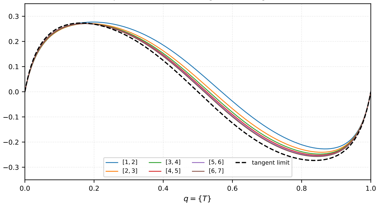
the pinned arches overlaid, against the tangent limit
