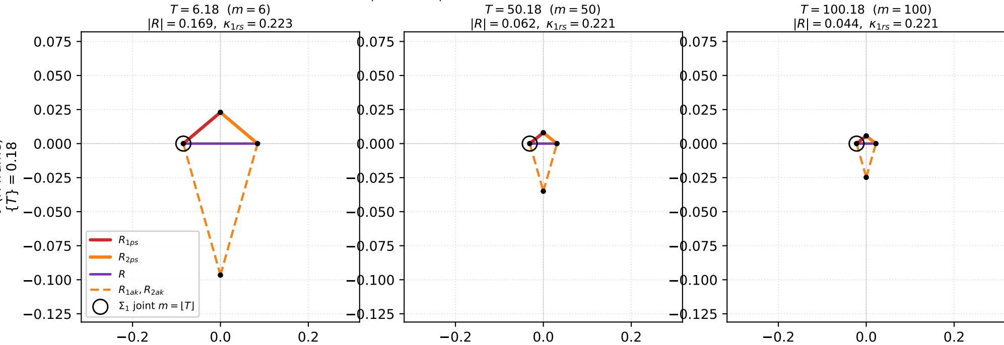
Remainders in the R -frame (center of R at the origin) at fixed \{T\} , varying [T] (common scale; R_{1ps} red, R_{2ps} orange, R purple, R_{1ak}+R_{2ak} orange dashed)
