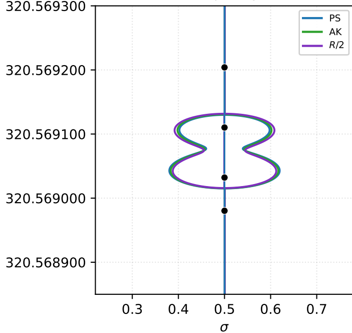
T \approx 320.57 : Equal legs ( L_1 = L_2 )
