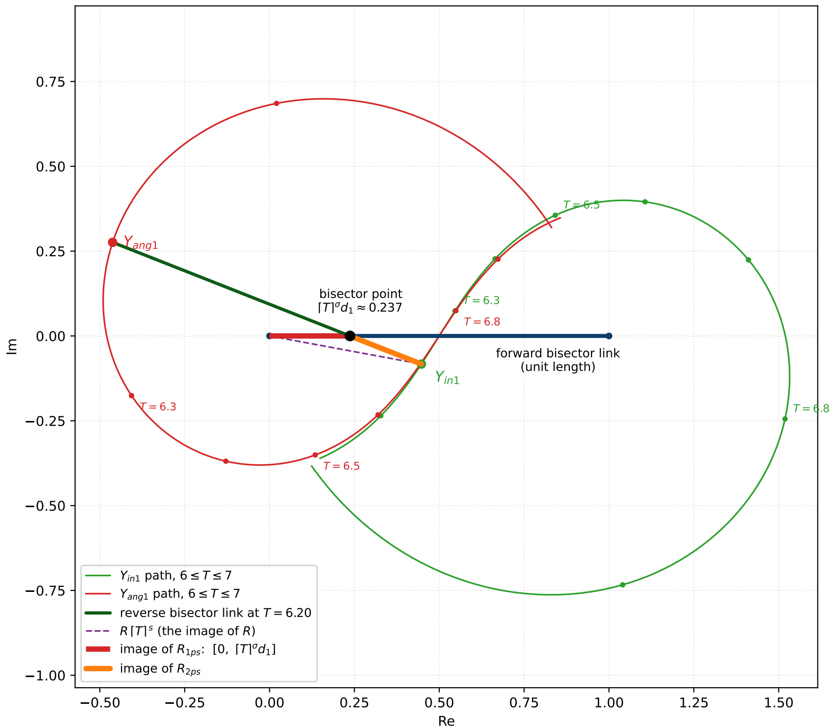
The yin and yang curves in the bisector frame ( \sigma = 1/4 , m = 6 )
