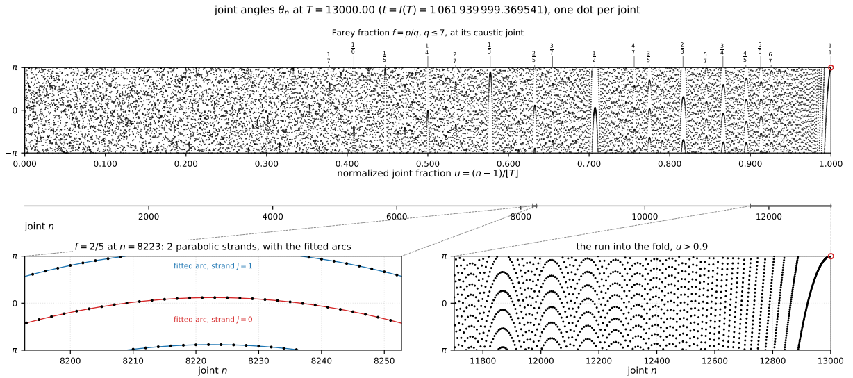
Figure 61: The joint-angle strip at T = 13000 , where t = I(T) = 1,061,939,999.369541 , one dot per joint of the forward chain, n = 2, \dots, [T] + 1 , with \theta_n of (211) on the vertical axis. The two edges \pm\pi are identified, so the strip is a cylinder. Top : all 13000 joints, carrying three horizontal scales: the Farey fractions f = p/q with q \leq 7 above, each at its caustic joint (212) and staggered in two rows where they crowd; the normalized joint fraction u = (n-1)/[T] below, so the bisector joint sits at u = 1 ; and the joint index n below that. The red circle at the right edge is the bisector joint n = [T] + 1 , where \theta = -\pi exactly. Bottom left : a window at f = \frac{2}{5} , showing its p = 2 parabolic strands as dots, each with its fitted arc (216) drawn through them; the two arcs sit half a turn apart, so strand 1 has its vertex wrapped to the opposite edge. Bottom right : the last tenth of the strip, where the strands steepen and run into that bisector joint on the right in the figure. Dashed lines carry each window back to the stretch of the joint- n scale it magnifies, marked there by a bracket. Generated by fig_joint_angles.py .
