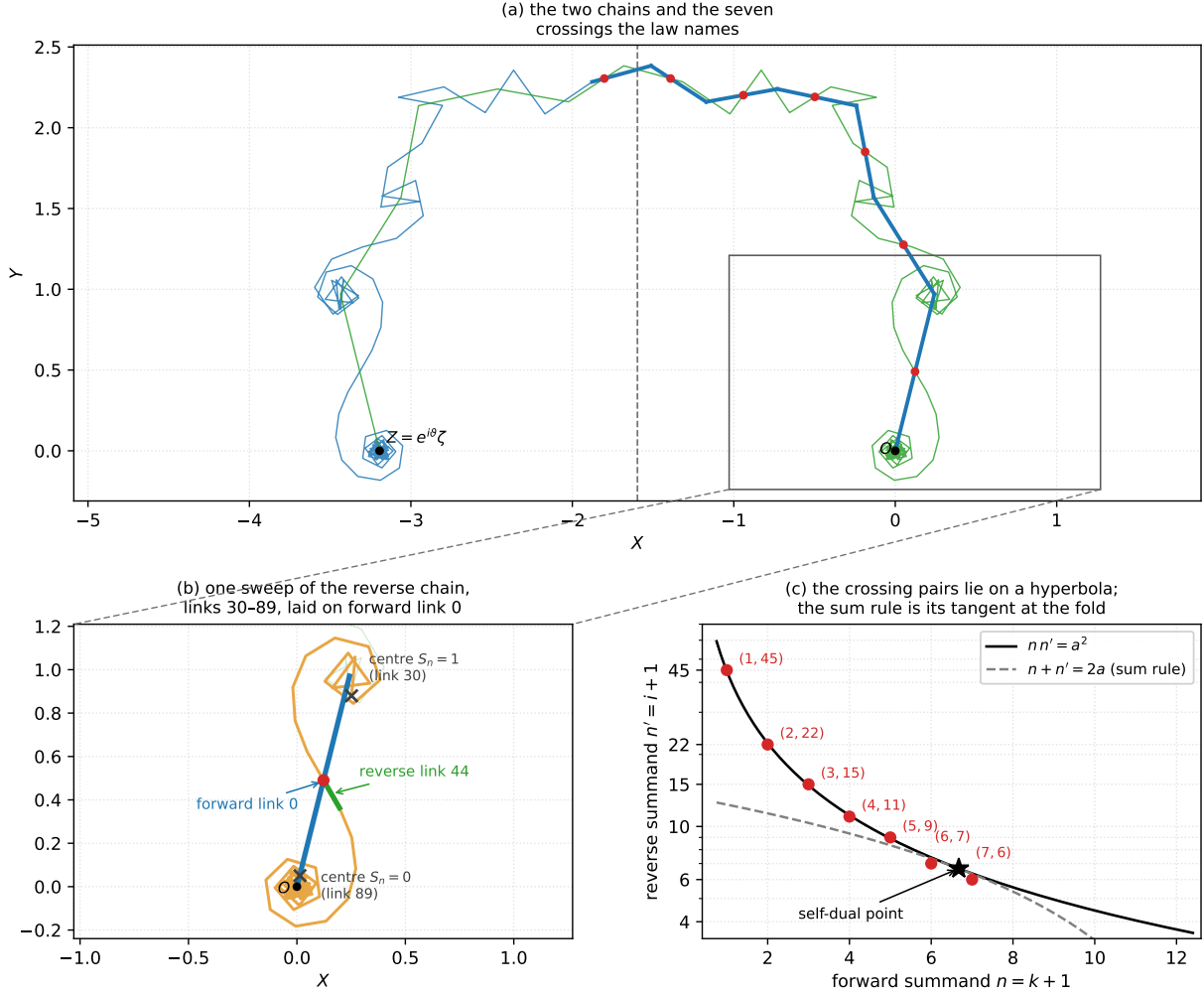
Figure 44: Links crossing at \sigma = \frac{1}{2} , T = 6.18 , the running example of Figure 2 ( t = I(T) \approx 279.85 , m = 6 , a = \sqrt{t/2\pi} = 6.674 , a^2 = 44.54 ; the first turn of each chain holds 90 links). (a) Both chains in the \vartheta -rotated frame, forward e^{i\vartheta}J_n in blue from O and reverse e^{i\vartheta}K_j in green from Z = e^{i\vartheta}\zeta , which by (137) is the blue chain reflected in the dashed bisector line X = Z/2 . Forward links 0 through 6 are drawn heavy and the red dots are the seven crossings (134) names for them, j = 44, 21, 14, 10, 8, 6, 5 ; they run the length of the chain, not just the neighborhood of the bisector. (b) The boxed region enlarged, showing why. The gold arc is one turn of the reverse chain, links 30 to 89, running from the spiral center S_n = 1 to the spiral center S_n = 0 (crosses, at the links (72) where the turn angle is an odd multiple of \pi ). By (141) that step reproduces forward link 0 reversed, so it lies back along the unit step and cuts it near the middle (red dot); the link carrying the sweep is 44, the middle of the turn, where the turn angle is 2\pi and n' = a^2/1 . (c) The pairs (n, n') of all seven crossings, on the hyperbola nn' = a^2 . The self-dual point n = n' = a (star) is the summand the law pairs about, half a unit of the index past T by (96). These are summand axes, and the star is plotted here at (a, a) with a = 6.674 , while the bisector link is link m = 6 , which carries summand n = 7 : the star therefore sits between summands 6 and 7, a third of a summand short of the bisector link's own value rather than past it. Near it the hyperbola is indistinguishable from its tangent n + n' = 2a (dashed), which is the sum rule (146), and away from it the two part company fast: the tangent gives the unit step a partner near n' = 11 where the truth is 45. Generated by fig_links_crossing.py .
