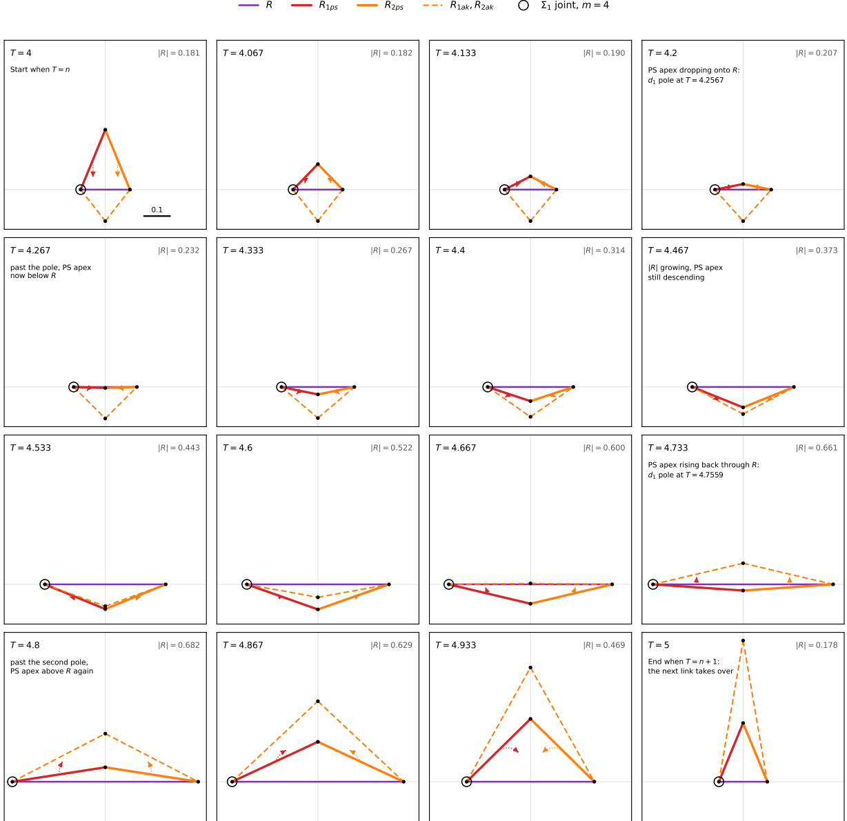
Figure 7: The remainder splits in the R -frame as T sweeps one unit, T = 4 \rightarrow 5 at \sigma = \frac{1}{2} , sixteen snapshots read left to right from the top left, the companion of Figure 32 for the remainders. The frame and the colors are those of Figure 6: R purple along the real axis with its midpoint at the origin, R_{1ps} red and R_{2ps} orange from the \Sigma_1 joint (open circle) to the far end of R , R_{1ak} and R_{2ak} orange dashed, all sixteen panels to one scale, with |R| given in each. The chain length is held at m = 4 throughout, as Figure 32 holds the bisector link constant, so T = 5 is the instant the handoff happens. The dotted arrow on R_{1ps} and on R_{2ps} runs from the middle of that segment to the middle of it as the next panel depicts it, tracing the motion between panels. Both apexes stay on the perpendicular bisector of R , the two halves of each split being equal in length on the critical line. The ps apex crosses the chord between the fourth and fifth panels and again between the twelfth and thirteenth, at the two heights of (63) where the split is the plain halving; the ak apex crosses once, between the tenth and eleventh. Generated by fig_remainder_frame_sweep.py .
