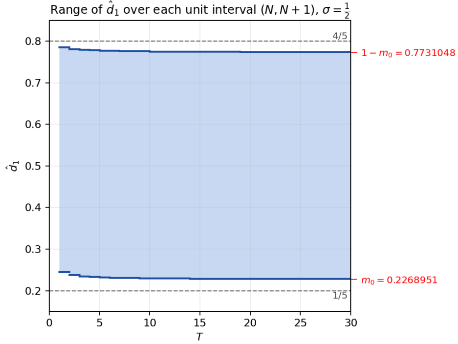
Figure 15: Range of the exact \hat{d}_1 over each unit interval (N, N + 1) , N = 1, \dots, 29 , on the critical line (blue bands; grid step 5 \times 10^{-4} for N < 3 , 10^{-3} after). Dashed black lines: the uniform bounds \frac{1}{5} and \frac{4}{5} of Theorem 8.12; the red right-hand scale marks the extremes m_0 = 0.2268951 \dots and 1 - m_0 = 0.7731048 \dots of the limit profile of Theorem 8.8. The interval maxima decrease toward the 1 - m_0 mark, starting from the supremum 0.78499 \dots attained on the first interval at T = 1.8530 \dots ; the interval minima decrease toward m_0 from above without attaining it. Generated by fig_interval_range.py .
