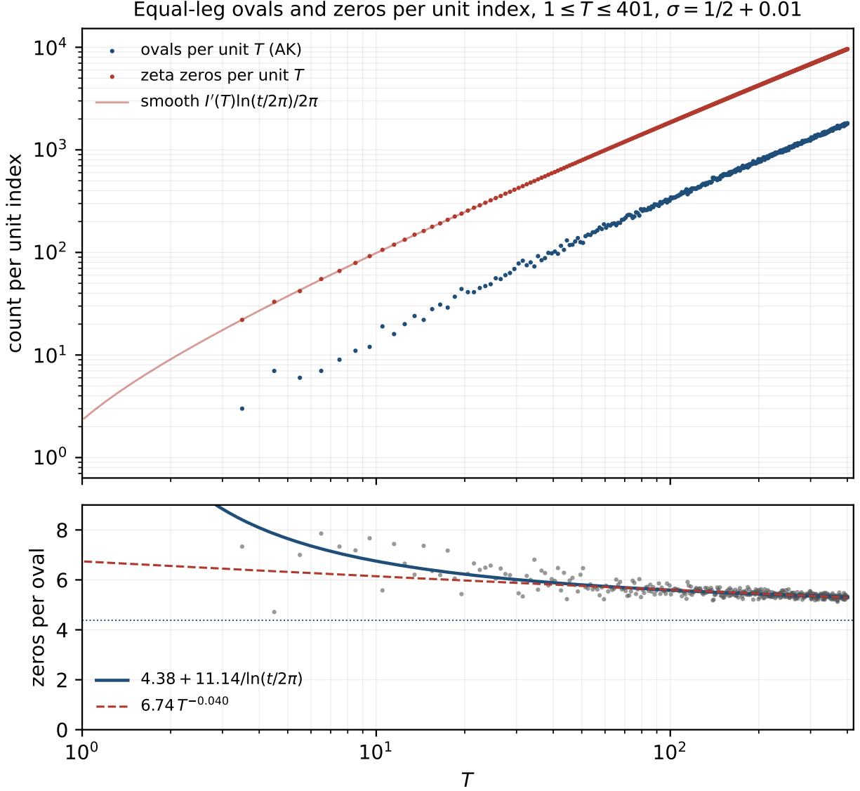
Figure 29: Above: equal-leg ovals and zeros of \zeta per unit interval of the index, 1 \leq T \leq 401 , at \sigma = \frac{1}{2} + 0.01 , log-log. The two clouds are parallel. Below: the interval's zeros per oval, with (92) solid and its limit 4.38 dotted, against the power law dashed. The two are indistinguishable over 50 \leq T \leq 400 and part company on either side. Generated by census_analyze.py of the equal-leg density companion note.
