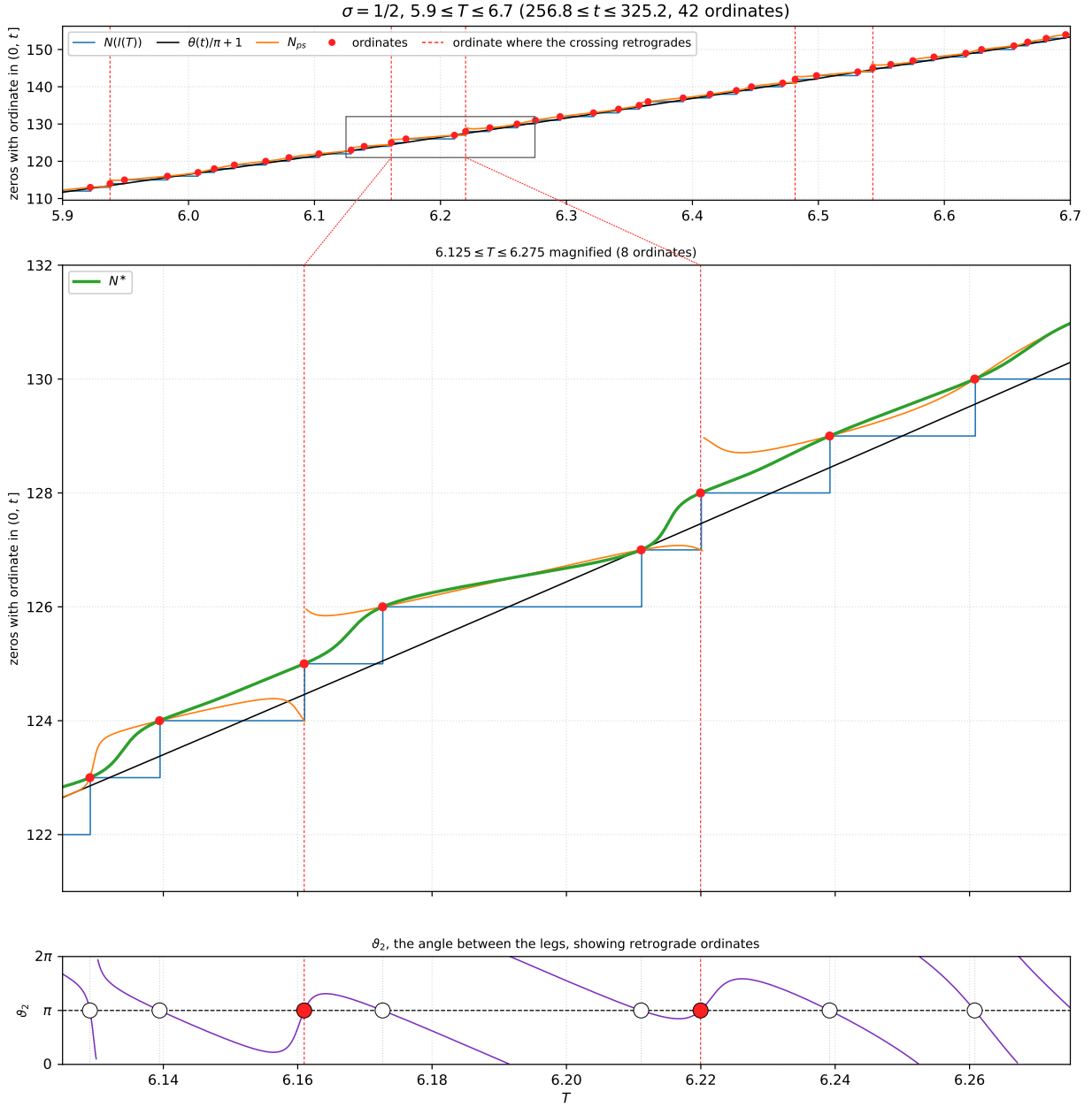
Figure 53: Staircase, in blue, is the exact Riemann–von Mangoldt formula (175), and the approximate Riemann–von Mangoldt formula (177) is the black curve, that formula with S dropped. Top : 5.9 \leq T \leq 6.7 , which is 256.8 \leq t \leq 325.2 and holds the 42 ordinates \gamma_{113} through \gamma_{154} , five of them retrograde, with N_{ps} of (178) in orange, broken at its wraps. Middle : the boxed window 6.125 \leq T \leq 6.275 magnified, holding 8 ordinates of which \gamma_{125} and \gamma_{128} are retrograde. The velocity split N^* of (185) is drawn in green. Bottom : the fold angle of the legs \vartheta_2 of §9.2 on the same T range, reduced to [0, 2\pi) . Every passage through \pi (dashed) is at an ordinate; the two filled dots are the two retrograde ordinates of the panel above, where \vartheta_2 rises through \pi , turns around, and comes back down through it. Generated by fig.nps_staircase.py .
