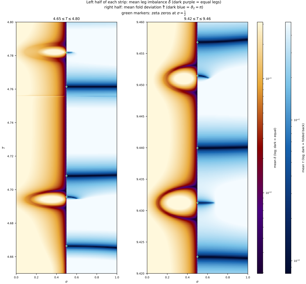
Figure 27: The two zoom windows of Figures 25 and 26 spliced at the critical line: in each strip the left half ( \sigma < \frac{1}{2} ) shows the mean leg imbalance \bar{\delta} of (86) on the color scale of Figure 25 (dark purple = equal legs), and the right half ( \sigma > \frac{1}{2} ) shows the mean fold deviation \bar{\tau} of (88) on the color scale of Figure 26 (dark blue = folded back). Both color maps are symmetric under \sigma \leftrightarrow 1 - \sigma (to a relative 10^{-10} on these grids), so each half carries its whole color map and the splice loses nothing. Green markers are zeta zeros. The length condition is dark along the seam and on the ovals flanking it; the angle condition is dark on the horizontal filaments; a zero is a filament reaching the seam. Generated by plot_leg_theta2_spliced.py .
