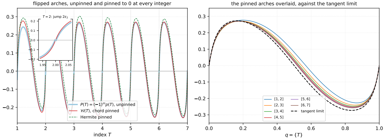
Figure 11: The flipped arches of p on the critical line, 1 \leq T \leq 7 . Left : the unpinned flip P of (56) (pale blue), which jumps by 2\varepsilon_n at each integer (inset, at T = 2 ); the chord-pinned \mathcal{W} of (57) (red), which is zero there exactly; and the Hermite-pinned variant (dashed green), which also matches the end slopes but inflates the arch. Right : the six pinned arches drawn against the fractional part q = \{T\} , with the tangent limit \mathcal{W}_\infty dashed; the deviation falls from 0.087 on [1, 2] to 0.025 on [6, 7] . Generated by fig_pinned_waveform.py .
