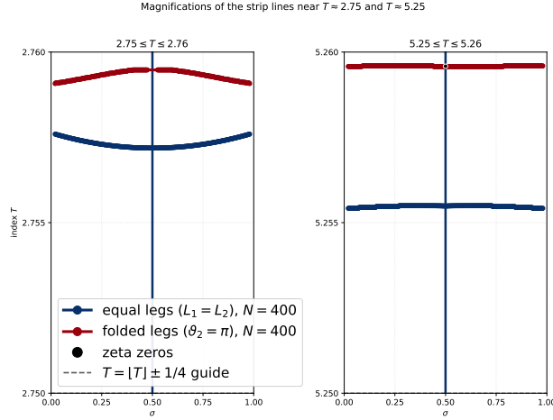
Figure 22: Two magnifications of the critical strip in the style of Figure 21: equal-leg locus L_1 = L_2 (blue) and folded-leg locus \vartheta_2 = \pi (red), each recomputed at N = 400 values of \sigma across (0, 1) ; critical line (blue vertical) and zeta zeros (black). Samples where the PS split is singular (tiny determinant) are omitted from the red locus, so the d_1 pole is not mislabeled as legs folded back. Left: 2.75 \leq T \leq 2.76 ; the blue equal-leg band sits near T \approx 2.757 and the red folded band near T \approx 2.759 , with a gap at \sigma = \frac{1}{2} (no zero in this window). Right: 5.25 \leq T \leq 5.26 ; blue near T \approx 5.255 and red near T \approx 5.2596 , meeting the critical line at the zeta zero in the window (not at the pole band). The dashed horizontal guide marks [T] \pm \frac{1}{4} ; the blue strip lines bow slightly across \sigma , symmetric about \sigma = \frac{1}{2} . At this resolution the red and blue loci do not cross off the critical line. Generated by fig-pole.heights.zoom.py .
