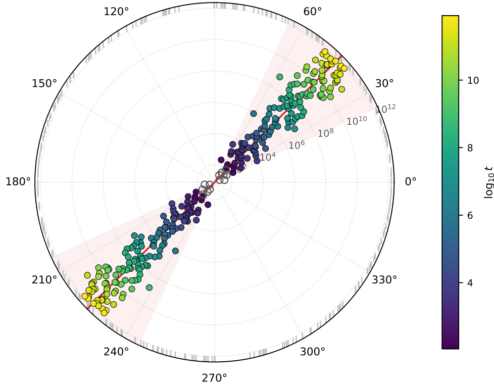
Figure 64: The last-link bearing (220) at the 148 champions above t = 17.8 , read at the nearest Gram point. The bearing is axial, so each champion is drawn at both ends of its axis; the radius is \log_{10} t , the color the height, the red line the circular mean and the shaded wedge \pm 20^\circ about it. Open circles are the six champions below t = 100 . The gray ticks around the rim are 148 ordinary Gram points over the same range of heights, whose bearings are uniform ( R = 0.052 ). The beam narrows outward: the tightest decade is the outermost, 10^{11} \leq t < 10^{12} , at R = 0.993 . Generated by fig_champion_bearings.py .
