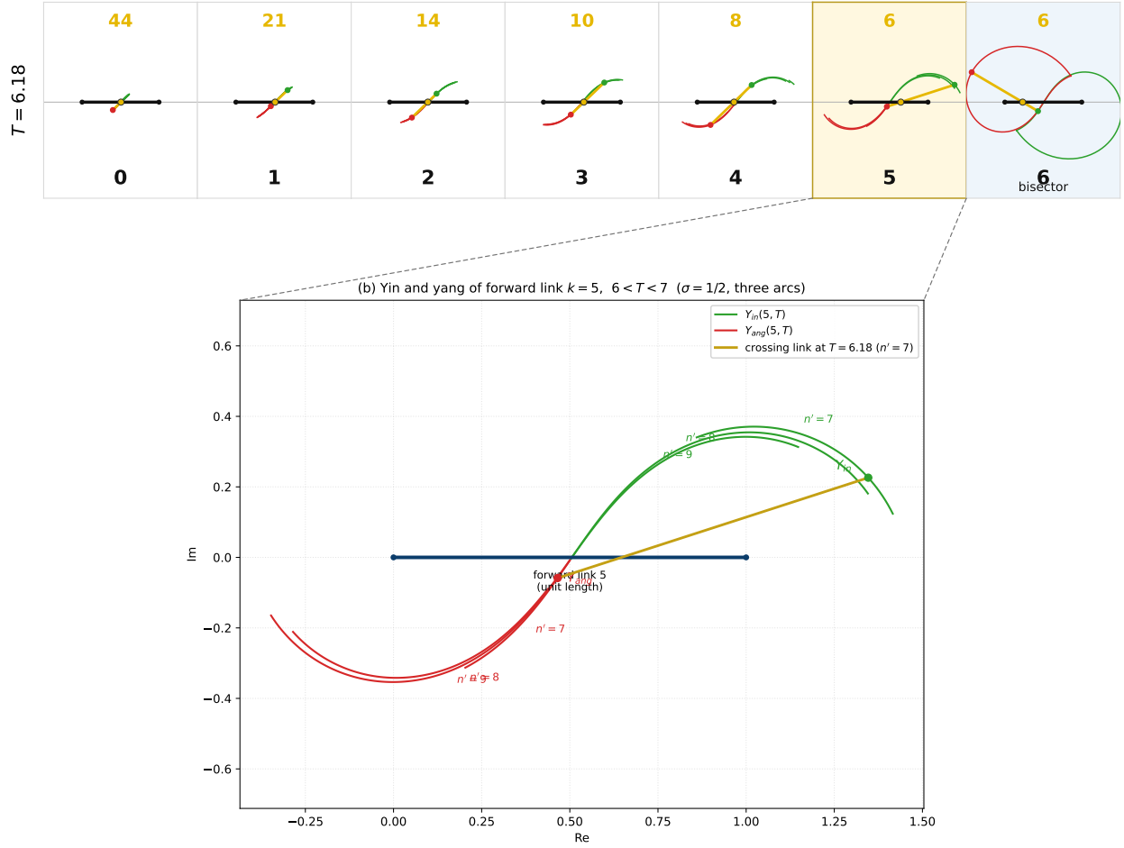
Figure 45: (a) Local frames of the forward links at \sigma = \frac{1}{2} , T = 6.18 , as in the top row of Figure 43, now with the yin and yang loci of every link as T runs through (6, 7) : green Y_{in}(k, T) , red Y_{ang}(k, T) . (b) The yin and yang curves of forward link k = 5 over 6 < T < 7 , from (151)–(154). The frame pins that link to [0, 1] (dark blue). Each end traces three arcs, one per crossing summand n' = 7, 8, 9 , kept apart where one reverse link gives way to the next: green is Y_{in}(5, T) , red is Y_{ang}(5, T) . The dark-yellow segment is the crossing link at the running example T = 6.18 , where C_\ell(5, 6.18) = 6 so n' = 7 . Dashed lines carry the local coordinate frame for link 5 of (a) down to the magnification (b). Each arc's yin is the previous arc's yang, the same joint passing from one reverse link to the next. Generated by fig-yinyang_link5.py .
