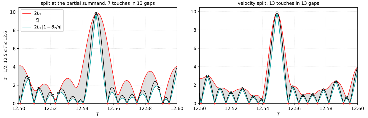
Figure 57: The two envelopes of (205), at \sigma = \frac{1}{2} , over 12.5 \leq T \leq 12.6 , the second window of Figure 55, which is 1061.3 \leq t \leq 1077.7 and holds 14 ordinates. In each panel |\zeta| is black, the upper envelope 2L_1 red, the lower envelope 2L_1|1 - \vartheta_2/\pi| a teal sawtooth, and the gray band between them is where |\zeta| is confined. Red dots on the axis are the ordinates, where the lower envelope touches zero along with |\zeta| , and the open circles are the touches of the upper envelope, one for each vanishing of the offset h . Left : the split at the partial summand, B_1 = \Sigma_1 + R_{1ps} , whose h fails to alternate at a retrograde ordinate, so it reaches its bound in only 7 of the 13 gaps and several humps rise nowhere near it. Right : the velocity split, whose h^* vanishes at every extremum of Z , so the upper envelope is touched in every gap. Generated by fig_envelope.py .
