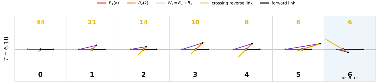
Figure 47: The cone (162) at \sigma = \frac{1}{2} , T = 6.18 , in the local frame of each forward link k = 0, \dots, 6 , the same local frames as the top row of Figure 45. Each local frame pins that link to [0, 1] on the real axis (black); the gold number is the reverse link that crosses it. Red is R_1(k) from the left joint to the crossing along the unit link, orange is R_2(k) from the crossing to reverse joint K_j , and purple is the resultant W_k . The last local frame is the bisector, W_6 = R . Generated by fig_Wk_triangle.py .
