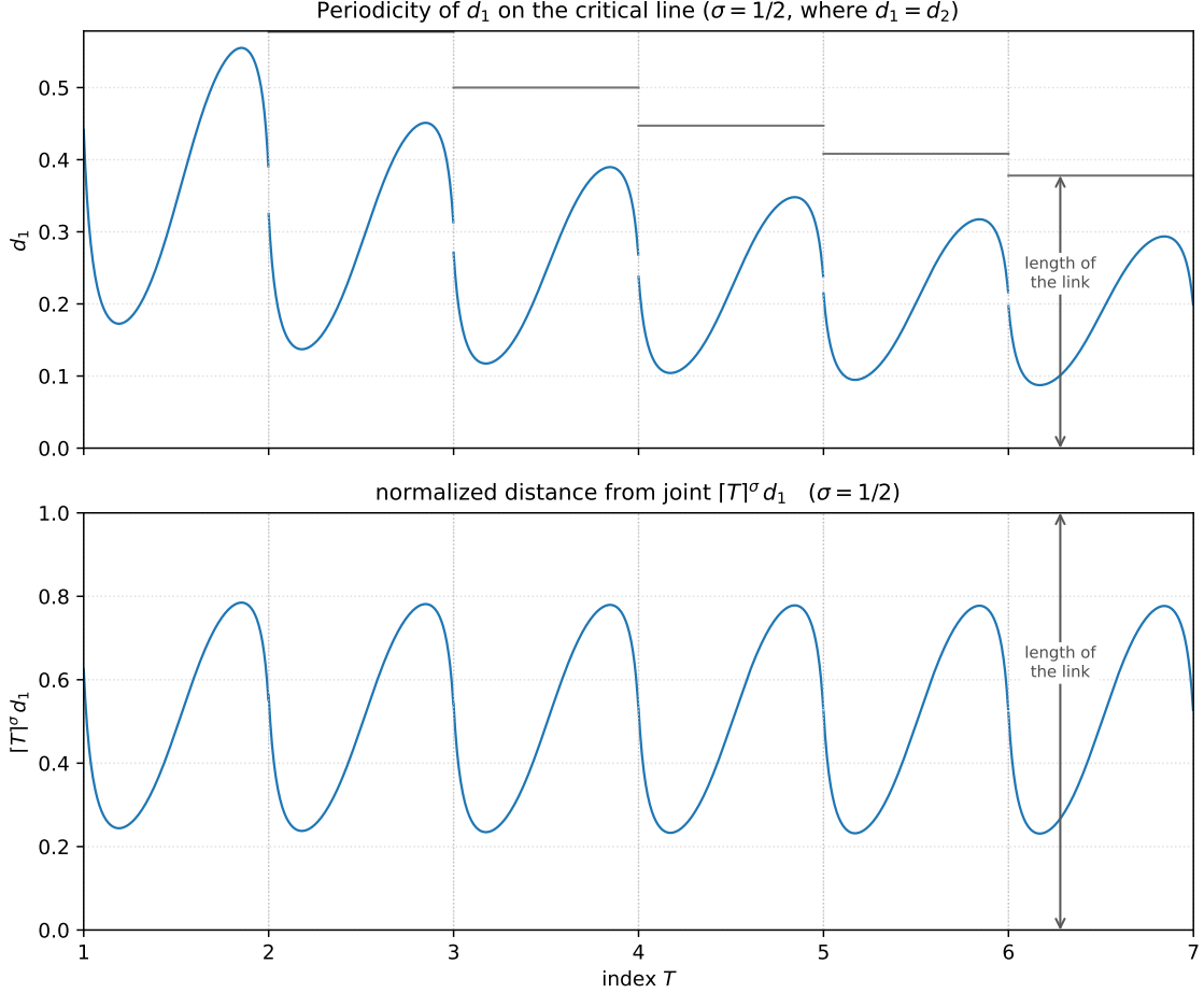
Figure 9: Top: the common fractional weight d_1 = d_2 on the critical line, plotted against the index T for 1 \leq T \leq 7 . The curve oscillates once per unit of T and jumps at each integer T , where m = \lfloor T \rfloor increments and the fractional summands hand off to the next link; the amplitude decays slowly as T grows. The gray step is the length [T]^{-\sigma} of the link that carries the fractional summand, which d_1 never exceeds; the panel keeps its original top, so the steps for 1 \leq T < 3 lie at or above the frame. The double-headed arrow on 6 < T < 7 spans that link length. Bottom: the same formula for d_1 normalized by the length [T]^{-\sigma} of link m , which carries it: the normalized distance from joint [T]^\sigma d_1 , the crossing fraction along link m at which the point B_1 = \Sigma_1 + R_{1ps} sits (cf. §11). The panel is drawn on the full scale 0 to 1 of the normalized link, so 0 is joint m and 1 is joint m+1 ; the double-headed arrow, at the same T as the one above, marks that same link seen at unit length. The normalization removes both the decay and (nearly) the jumps: the fraction sweeps the same range \approx [0.23, 0.78] in every unit interval, staying clear of both ends of the link (made exact in §8.6–§8.7). So the normalized curve converges to a periodic waveform: sampled at matched fractional parts of T , its values agree to \approx 2 \times 10^{-3} by T = 20 , and the residual discrepancy halves with each doubling of T , the rate set by the link-length mismatch (1 + 1/\lfloor T \rfloor)^\sigma \rightarrow 1 of (51) below. Computed exactly (mpmath) via the Cramer solution of (23). Generated by fig.d1_critical.py .
