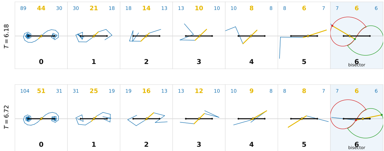
Figure 43: Local frames of the forward links at \sigma = \frac{1}{2} , T = 6.18 (top) and T = 6.72 (bottom), the running example of Figure 2 and a later height in the same unit ( t = I(T) \approx 279.85 and 327.01 , m = 6 ). Each panel is the local coordinate frame for that forward link, by pinning one forward link to the unit interval along the x -axis; the number at the bottom is that link. The reflected reverse chain is drawn in the same frame: the blue links are the part of it that belongs to the particular forward link, numbered at the two ends with the outer (higher) link on the left, and the yellow link is the single reverse link that crosses the forward link, numbered in yellow, with a yellow dot at the crossing. The rightmost local frame is the bisector; the green and red curves are the yin and yang loci of the two ends of the reverse bisector link as T runs through (6, 7) . Generated by fig.link_frames.py .
