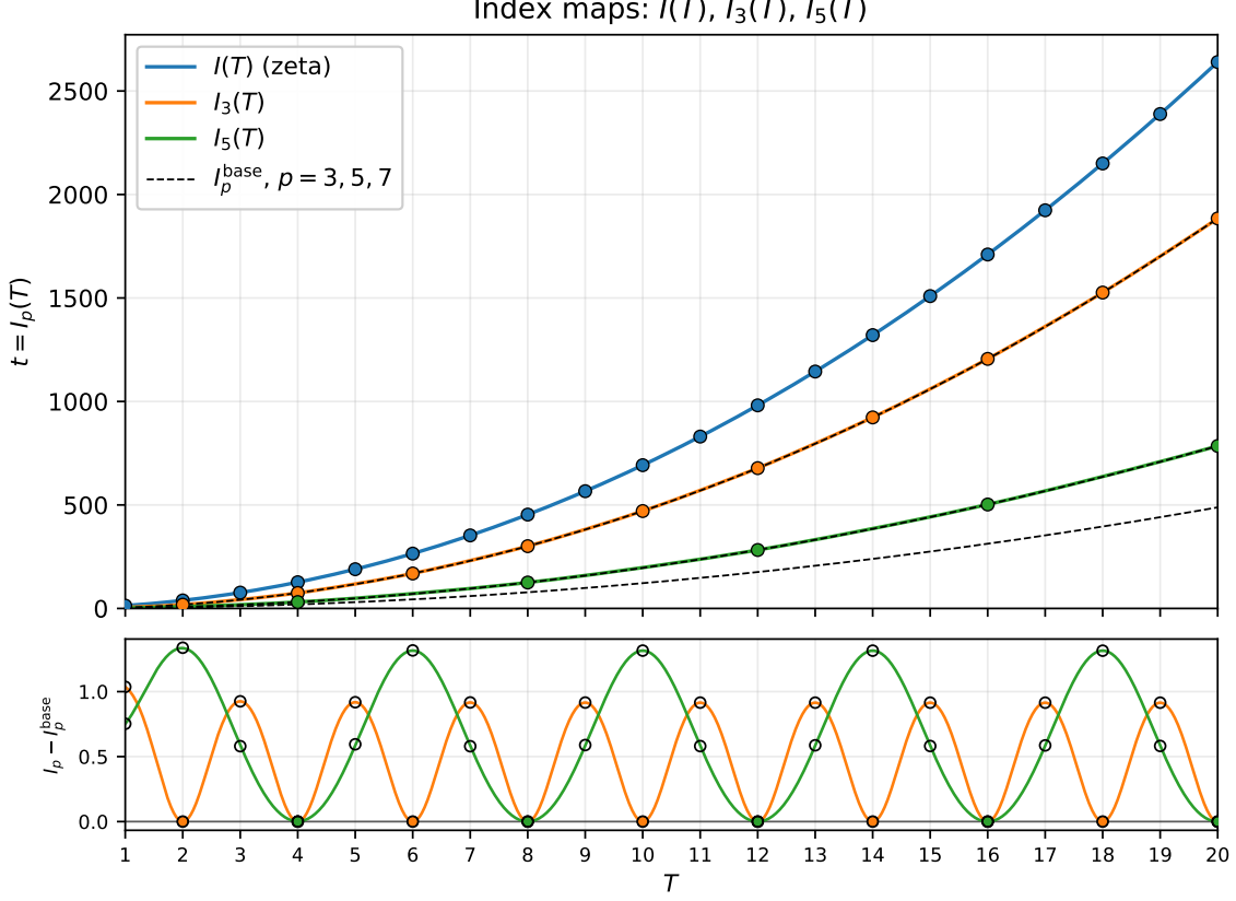
Figure 35: Top: index maps on T \in [1, 20] : zeta's I(T) (blue), I_3(T) for p = 3 (orange), and I_5(T) for p = 5 (green). Dots mark the fold events, at T \equiv 0 \pmod{p-1} : every integer on the zeta curve, every other integer on I_3 , and every fourth integer on I_5 . Leading growth is quadratic with coefficients 2\pi , \frac{3}{2}\pi , and \frac{5}{8}\pi respectively. Thin dashed black: the smooth base maps (98) for p = 3, 5, 7 . The p = 3 and p = 5 bases are hidden under I_3 and I_5 at this scale; the p = 7 base is the lowest curve, drawn for comparison, no I_7 having been fitted here. Bottom: the character bulge on its own scale, I_p - I_p^{\text{base}} , which the top panel cannot resolve because it is of order 1 against values in the thousands. It is one-signed, returning to zero at the folds (dots) and rising to \approx 0.92 between them for p = 3 and \approx 1.33 for p = 5 , and its amplitude barely decays: the p = 3 peaks are 0.9253, 0.9183, 0.9153 at T = 3, 5, 11 . So the correction is a fixed additive offset, not a fixed relative one. Open black circles are the numerically scanned events at every integer T , measured against the same base: the folds sit on zero, the intermediate events ride the bulge, and all of them follow the modeled curves to within 1.7 \times 10^{-5} for p = 3 and 1.0 \times 10^{-2} for p = 5 on T \leq 20 . Generated with the Dirichlet L -function companion note.
