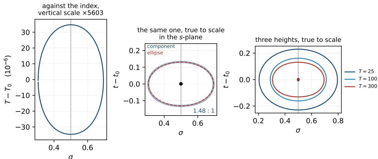
Figure 28: Why the components of the equal-leg locus are called ovals. Left: one of them at T = 300 plotted against the index, as the strip figures plot them, the vertical axis stretched by 5600 to make it visible. Middle: the same component in the s -plane with the axes to a common scale, and the ellipse through its extremes dashed over it; the dot is the zero of \zeta it encloses. Right: components at T = 25, 100 and 300 to a common scale, each drawn about its zero. They shrink with height and hold their shape. All three are the median-height component of their interval, taken among those whose zero sits nearest the middle, since the zero is central only on average. Generated by fig_oval_shape.py of the equal-leg density companion note.
