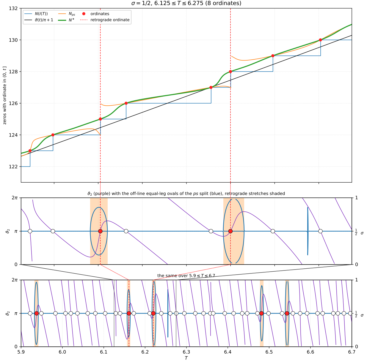
Figure 56: The count, the fold angle, and the equal-leg locus of the ps split read together, everything at \sigma = \frac{1}{2} except the locus. Top: the magnified window 6.125 \leq T \leq 6.275 of Figure 53: the staircase (blue), the smooth part (black), N_{ps} (orange), N_* (green), and the retrograde ordinates dashed in red. Middle: \theta_2 on the same window (purple), reduced to [0, 2\pi) and broken at its wraps, with the equal-leg locus L_1 = L_2 of the ps split drawn in the surrounding strip (blue) on the shared vertical scale 2\pi\sigma , \sigma on the right-hand axis. The horizontal blue line on the dashed \theta_2 = \pi line is the critical line, which belongs to the locus at every height; the two blue ovals are the off-line components in this window. Dots mark the ordinates, where \theta_2 passes through \pi , filled red at the retrograde ones; the shaded stretches are where \theta_2 runs retrograde. Each oval fills a shaded stretch and each stretch holds one retrograde ordinate. The thin blue band at T \approx 6.255 is the pole band of Figure 19 at \{T\} \approx \frac{1}{4} , not an oval. Bottom: the same reading over the full window 5.9 \leq T \leq 6.7 of Figure 53: five retrograde stretches, five ovals, and the five retrograde ordinates. Generated by fig_count_theta2_ovals.py .
