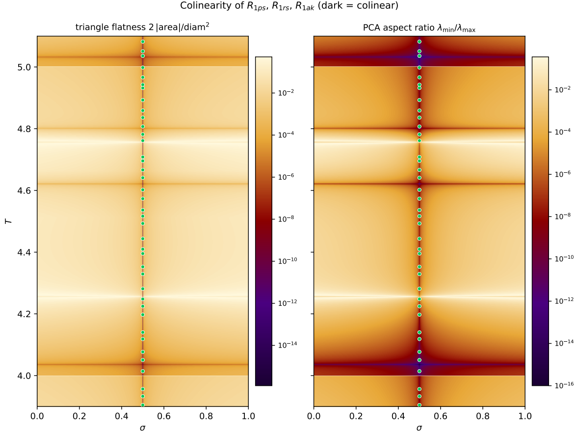
Figure 59: Collinearity of the three first-half remainders R_{1ps} , R_{1rs} = \frac{1}{2}R , R_{1ak} (dark = collinear). Horizontal axis \sigma \in [0, 1] ; vertical axis the spiral index T \in [3.9, 5.1] . Left: triangle flatness (209); right: PCA aspect ratio \lambda_{\min}/\lambda_{\max} . Both panels use a log color scale; green markers are zeta zeros at \sigma = \frac{1}{2} . The dark column pinned at the numerical floor along \sigma = \frac{1}{2} shows the three points are exactly collinear everywhere on the critical line; off the line collinearity occurs only along the isolated dark horizontal bands. Generated by fig_collinearity_zoom.py from data produced by remainder-collinearity-heatmap-zoom.mjs .
