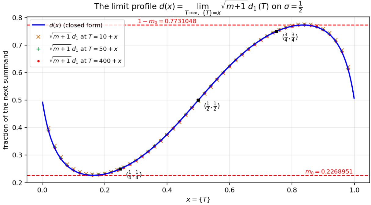
Figure 14: The closed-form profile d(x) of Theorem 8.8 (blue) against the exact \sqrt{m+1} d_1 sampled at T = 10 + x , 50 + x , 400 + x on the critical line. Already at T = 10 + x the samples sit on the curve; the marked squares are the exact values (\frac{1}{4}, \frac{1}{4}) , (\frac{1}{2}, \frac{1}{2}) , (\frac{3}{4}, \frac{3}{4}) , and the dashed red lines are the extremes m_0 = 0.2268951\dots and 1 - m_0 = 0.7731048\dots of the profile. Generated by fig_d_limit.py .
