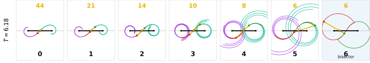
Figure 46: Local frames of the forward links at \sigma = \frac{1}{2} , T = 6.18 , as in panel (a) of Figure 45, with each non-bisector yin and yang arc continued as a solid curve (teal past the green end farther from the origin, purple past the other red end). The continuation holds the reverse link of that piece and runs half a unit of T . The bisector local frame is not extended. Generated by fig_yinyang_extended.py .
