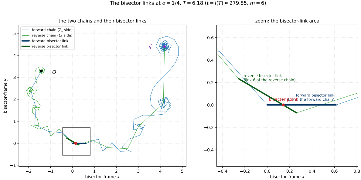
Figure 36: The two bisector links at \sigma = \frac{1}{4} , T = 6.18 ( t = I(T) \approx 279.85 , m = 6 ). Both panels are drawn in the coordinate frame of the forward bisector link : the whole picture is translated and rotated so that this link lies along the positive x -axis, with no rescaling. All lengths are true, so the link runs from 0 to 7^{-1/4} \approx 0.615 . Left : the forward chain (blue, starting at the world origin O ) and the reverse chain (green, ending at \zeta ), each drawn out to the link nearest its spiral center; link 6 of each chain (the forward and reverse bisector links) is overdrawn with a thick stroke, and the red dot where they cross is the bisector point. Right : zoom into the gray window: the two bisector links crossing at the bisector point, which sits on the x -axis at distance d_1 from the origin. The bisector frame of this section additionally rescales this link to the unit interval [0, 1] and watches the thick reverse link revolve around it. Generated by fig_yinyang_spirals.py .
