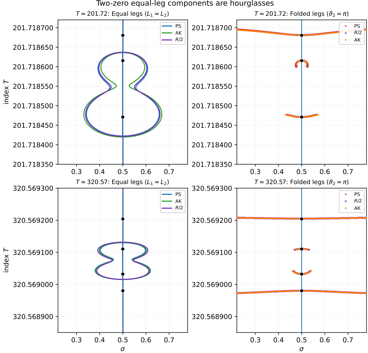
Figure 31: Two AK ovals that each enclose two zeros, drawn as in Figure 23. Top: the first such oval, at T \approx 201.72 . Bottom: another at T \approx 320.57 . Left: equal-leg loci L_1 = L_2 for PS (blue), AK (green), and R/2 (purple). Right: folded-leg loci \theta_2 = \pi for the same three choices (red, orange, and hollow purple). The blue vertical is the critical line; black dots are zeta zeros. Each equal-leg component is an hourglass, two oval lobes joined at a neck, with one zero in each lobe. The three splits nest and keep that shape. Generated by fig_two_zero_hourglass.py .
