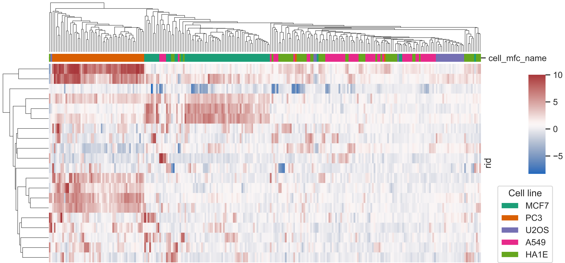
Clustering of Top Variable Genes Across Signatures
