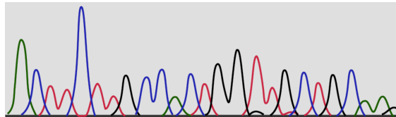
Figure 5: Draven Electropherogram
