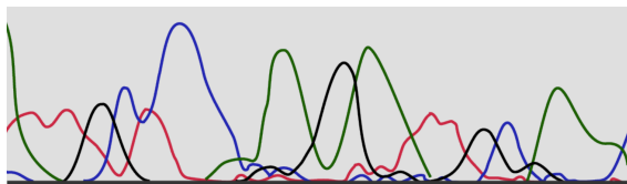
Figure 4: Katarina Electropherogram
