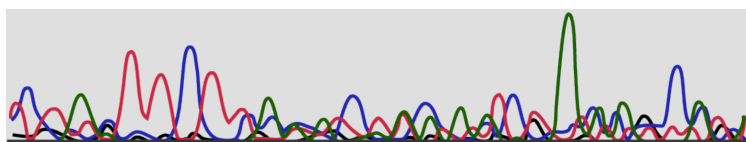
Figure 6: Yuumi Electropherogram
