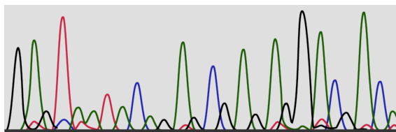
Figure 2: Teemo Electropherogram
