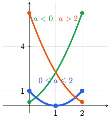
moving axis a on 0 \leq x \leq 2
