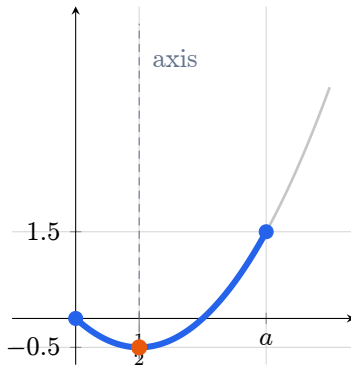
moving endpoint a
