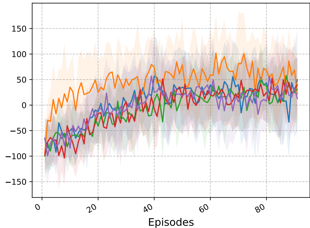
HalfCheetah-v4
