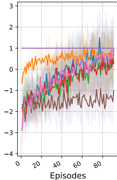
HalfCheetah-v4
