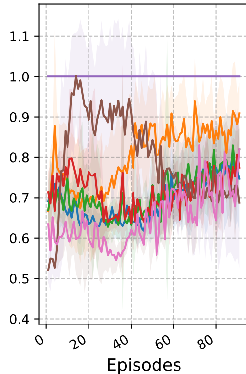
Hopper
