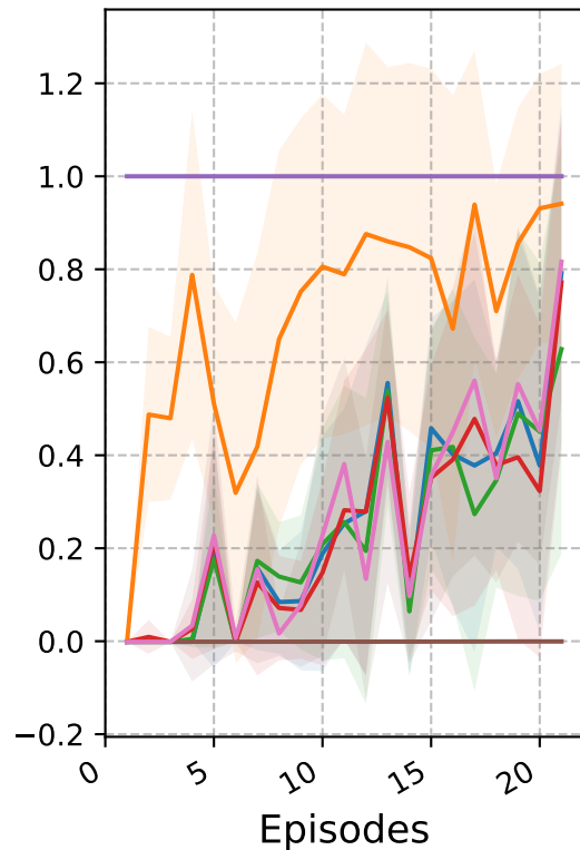
MountainCarContinuous-v0
