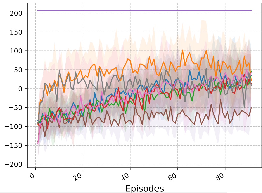
HalfCheetah-v4
