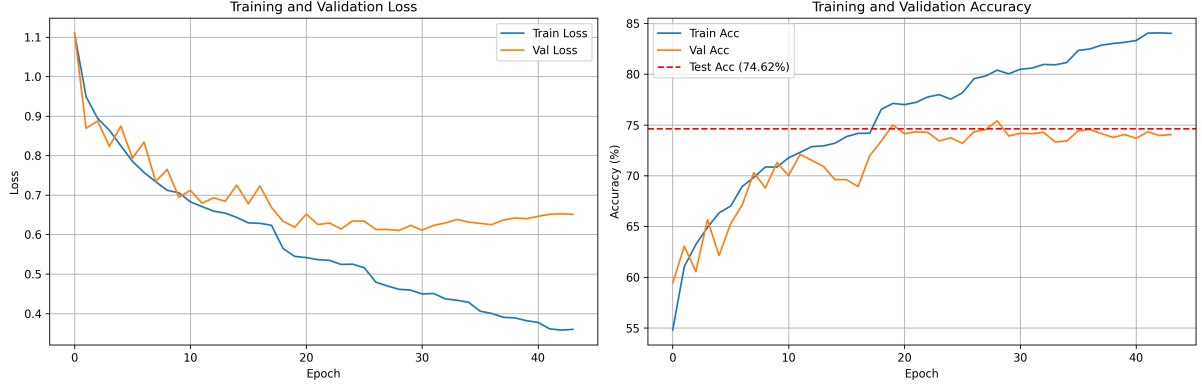
Figure 1: ResNet18-BiLSTM training history (44 epochs). Left: cross-entropy loss; Right: accuracy. Validation accuracy plateaued around epoch 35, triggering early stopping at epoch 44. Final test accuracy: 74.6%.
