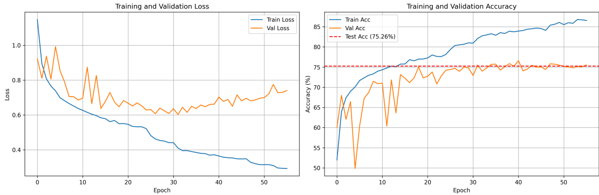
Figure 2: MobileNet-LSTM training history (56 epochs). Left: cross-entropy loss; Right: accuracy. The model converged more gradually than ResNet18-BiLSTM and achieved a higher test accuracy of 75.3%, making it the selected deployment model.
