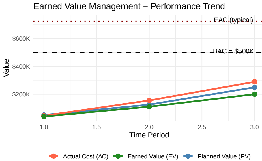
Figure 5.1.: EVM trend chart. When EV falls below PV, you're behind schedule. When AC rises above EV, you're over budget. Both conditions here — a project in the red on both dimensions.
