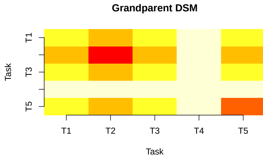
Figure 8.2.: Grandparent DSM heatmap. Shows risk-based coupling: tasks that share risk exposure through common resources tend to fail together.
