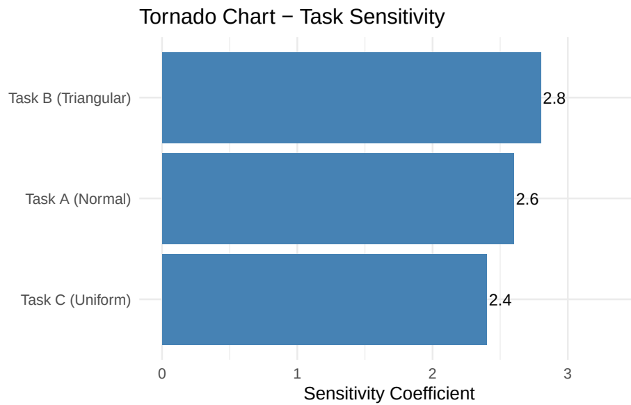
Figure 2.2.: Tornado chart showing each task's contribution to total schedule variance. Focus risk mitigation on the tallest bars.
