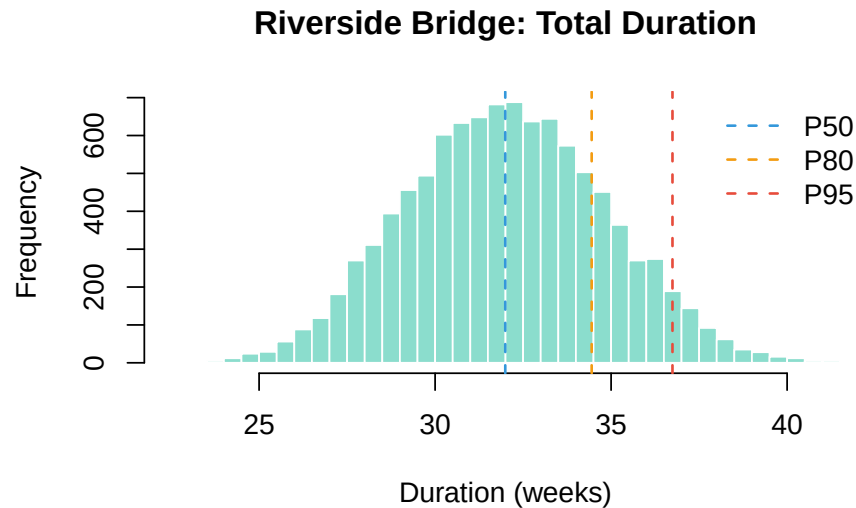
Figure D.1.: Total project duration distribution. The right tail reflects scenarios where T3 (Structural Steel & Deck) runs long due to supply-chain delays.
