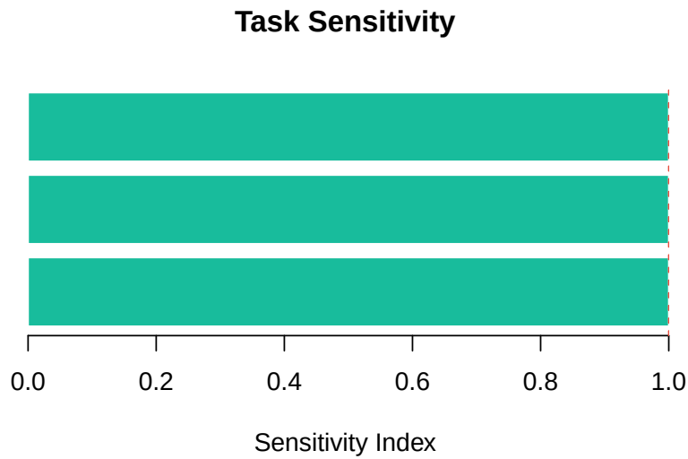
Figure 4.1.: Tornado chart of task sensitivity indices. The tallest bar is the dominant risk driver — the task where reducing variance has the greatest effect on total project uncertainty.
