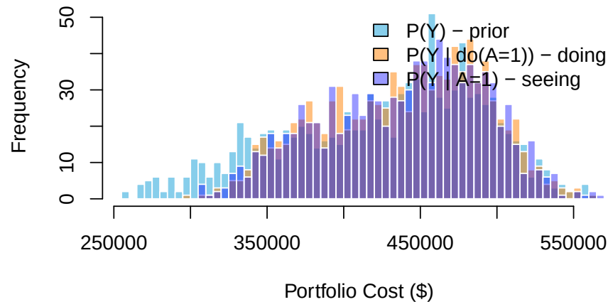
Figure 10.3.: Prior, doing, and seeing distributions for portfolio cost. Seeing shifts further right than doing because it propagates through the shared root cause SC.
