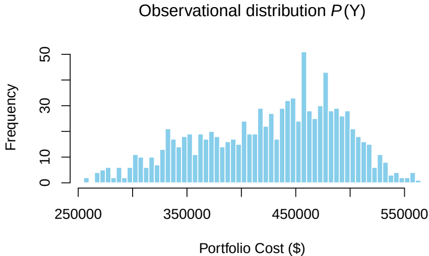
Figure 10.1.: Observational portfolio cost distribution P(Y) . Heavy tails reflect compounded shared-risk uncertainty.
