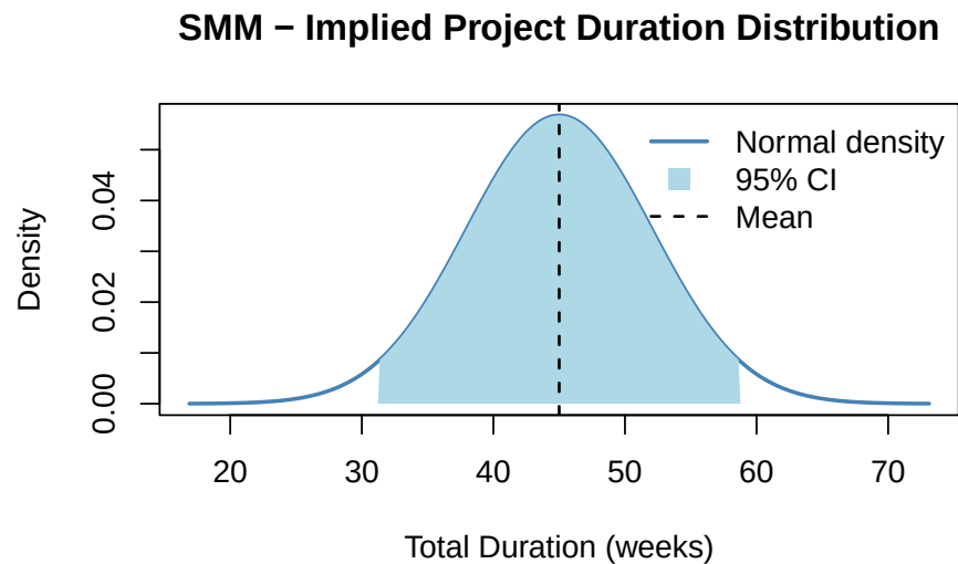
Figure 3.1.: SMM implied normal distribution for total project duration. The shaded region is the 95% confidence interval.
