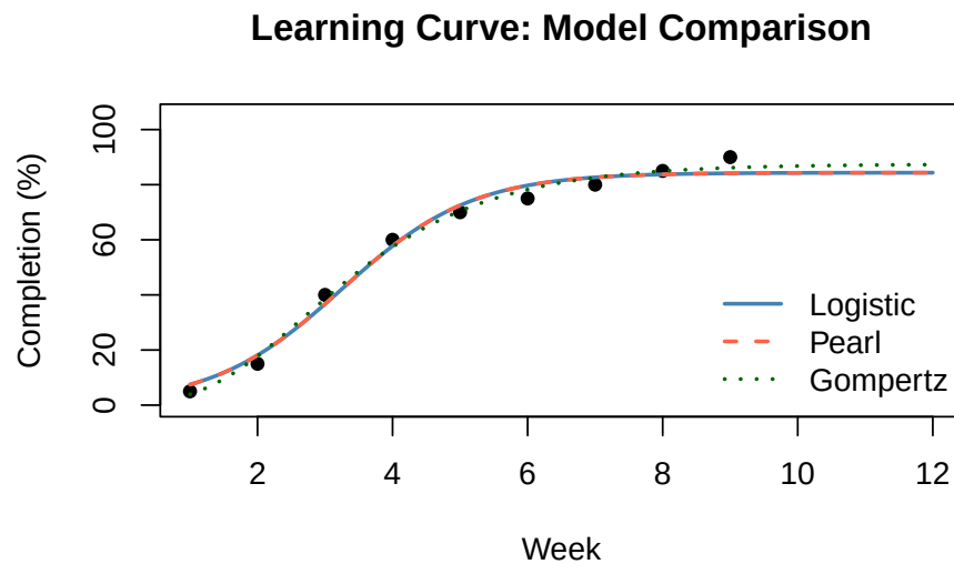
Figure 7.2.: Comparison of Logistic, Pearl, and Gompertz fits. Logistic and Pearl are identical; Gompertz has a different early-acceleration shape.
