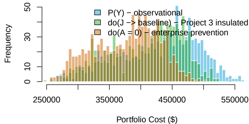
Figure 10.4.: Project-scoped vs. enterprise-level labor risk mitigation. Enterprise prevention eliminates exposure across all three projects.
