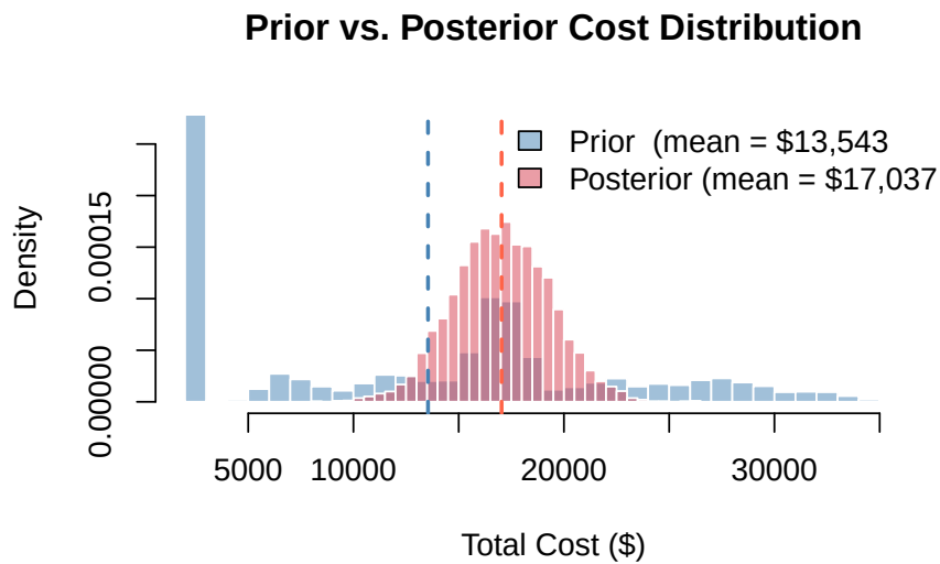
Figure 6.2.: Prior vs. posterior cost distribution. Confirming which risks materialized narrows and shifts the distribution.
