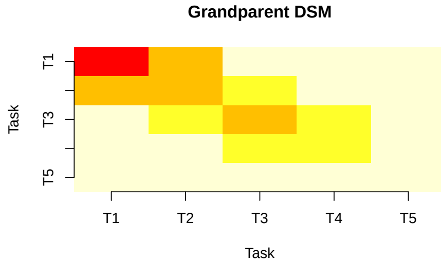
Figure D.5.: Grandparent DSM (risk-based coupling). Ground Conditions risk creates coupling between T1–T2 through the shared Civil Engineer and Survey Crew resources.
