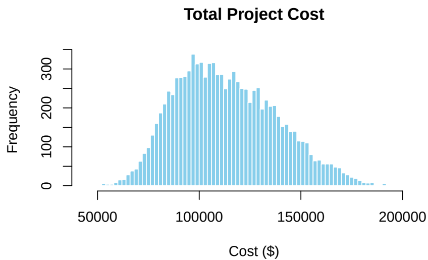
Figure 9.1.: Total project cost distribution from 10,000 forward simulations. The right tail represents scenarios where both risks occur simultaneously.
