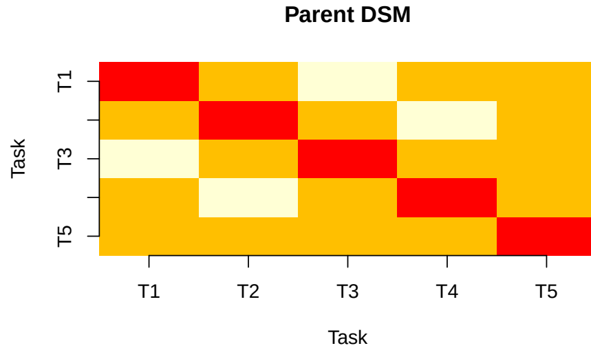
Figure 8.1.: Parent DSM heatmap. Darker cells indicate more shared resources between tasks — and therefore more potential for correlated disruption.
