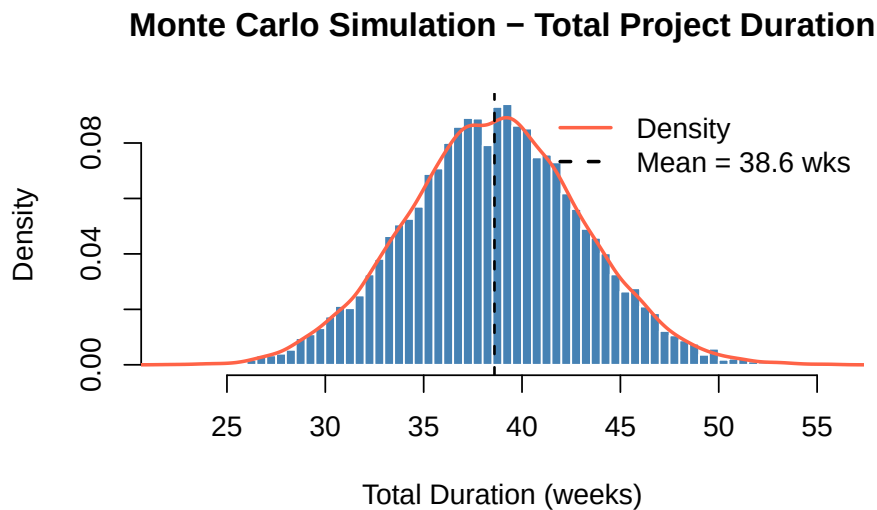
Figure 2.1.: Monte Carlo simulation results showing the full distribution of possible total project durations.
