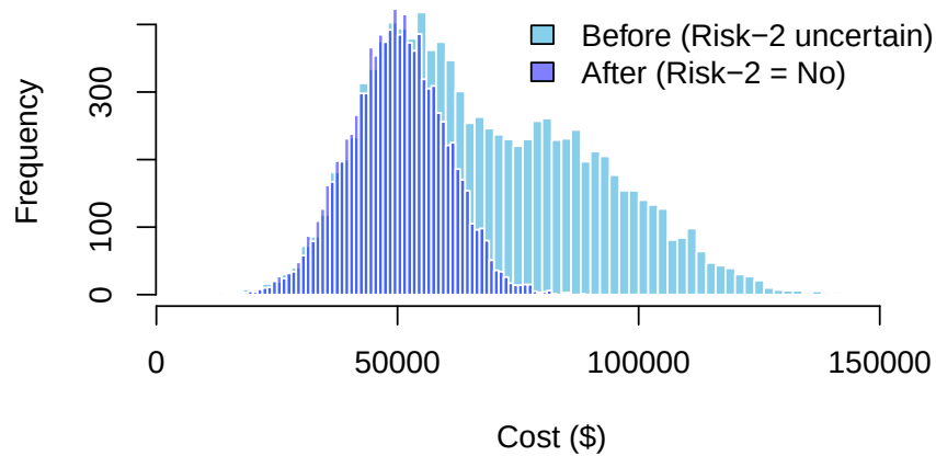
Figure 9.2.: Developer cost before and after observing Risk-2 = No. The distribution collapses to the lower baseline.
