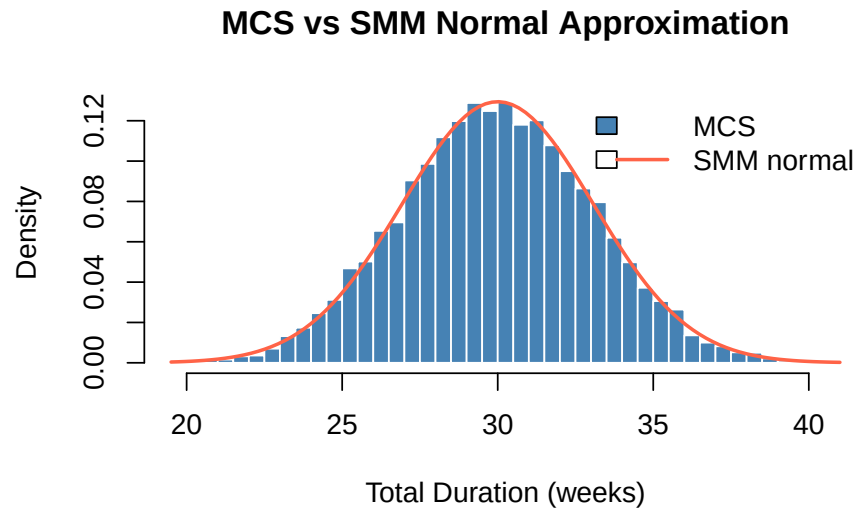
Figure E.1.: SMM normal approximation (red curve) overlaid on the MCS histogram. The fit is good for this 3-task project; the slight right skew from Task B is the main deviation.
