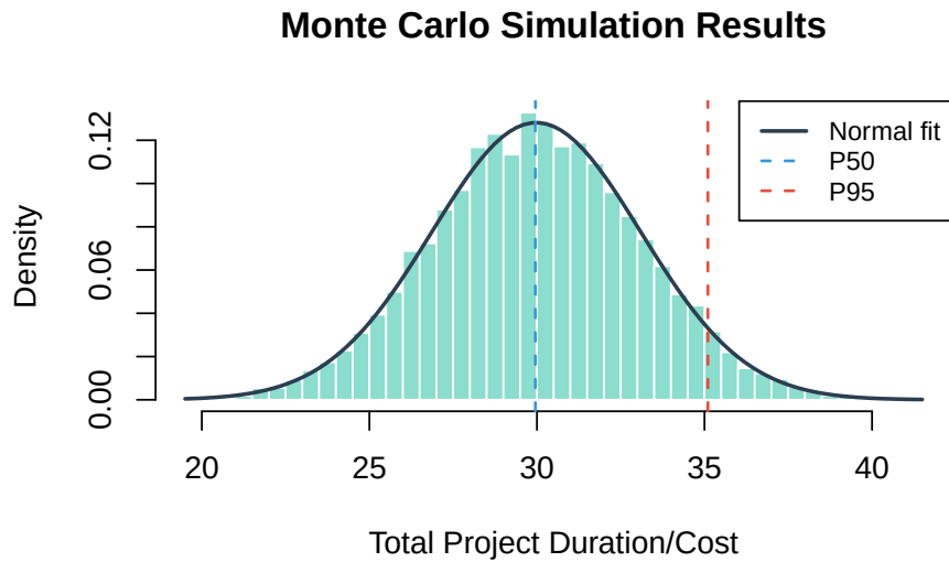
Figure 11.1.: MCS results via slash command. The /mcs command stores results for downstream chaining.
