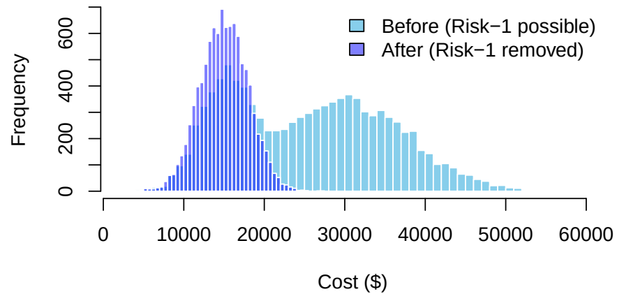
Figure 9.3.: Business Analyst cost before and after removing the Risk-1 arc. The heavy right tail disappears.
