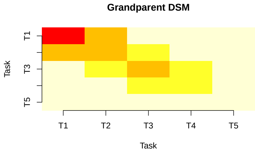
Figure A.5.: Grandparent DSM (risk-based coupling). Ground Conditions risk creates coupling between T1–T2 through the shared Civil Engineer and Survey Crew resources.
