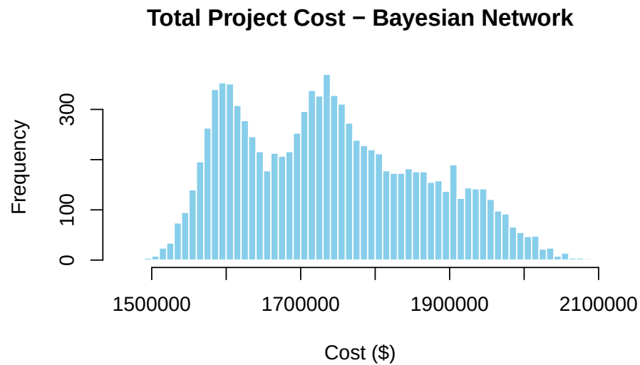
Figure A.6.: Total project cost distribution from the Bayesian network. The bimodal shape reflects whether ground conditions risk materialises.
