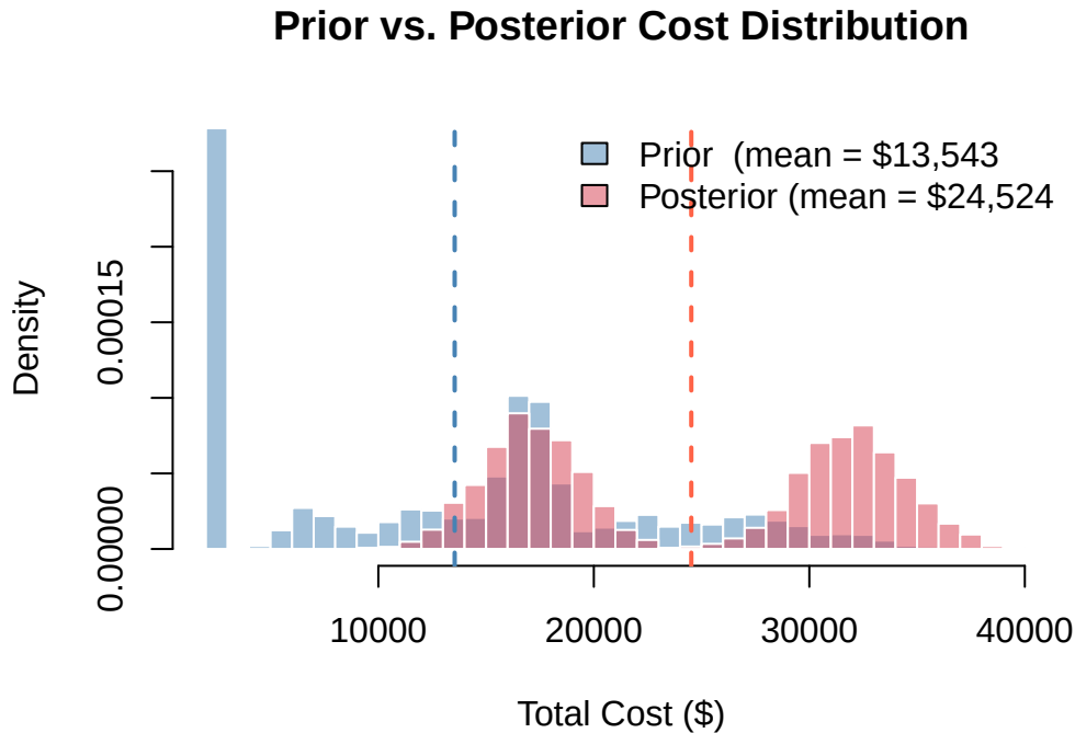
Figure 6.3.: Prior vs. posterior cost distribution. Confirming which risks materialized narrows and shifts the distribution.
