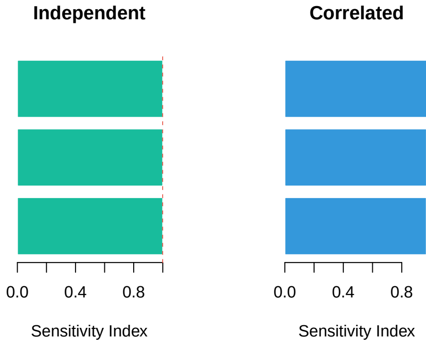
Figure 4.2.: Sensitivity indices when tasks are correlated. Positive correlations amplify the dominant driver (Task A) and increase total project variance.
