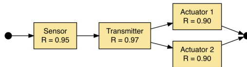
Figure 2.3: Mixed RBD: Sensor–Transmitter in series, Actuators 1 & 2 in parallel
