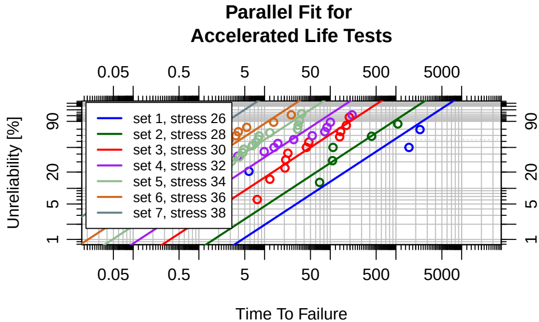
Figure 7.14: Interactive Power Law–Weibull ALT probability plot (electrical insulating fluids)
