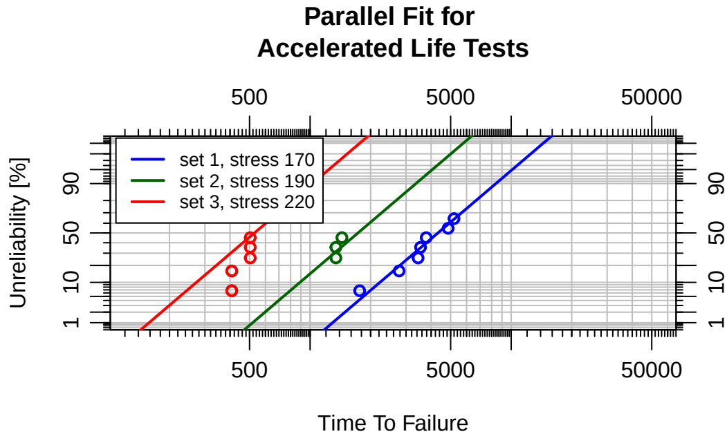
Figure 7.10: Interactive ALT probability plot: Arrhenius-Lognormal model (Class B insulation)
