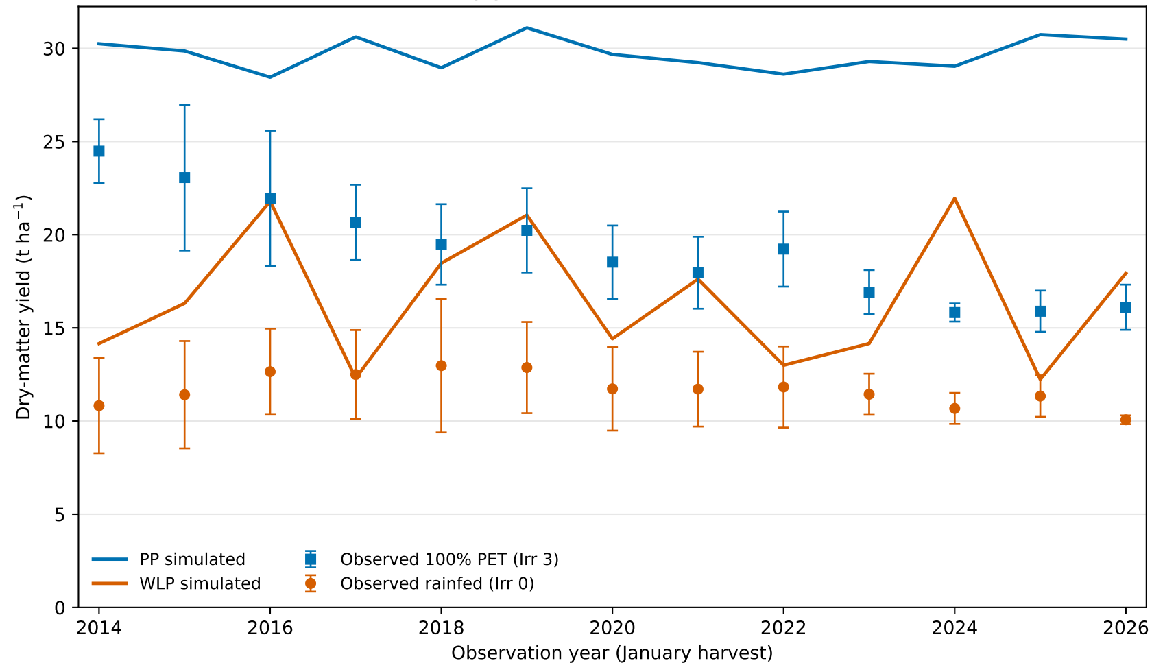
WOFOST Miscanthus × giganteus Yield: Simulated vs Observed (Aliartos)
