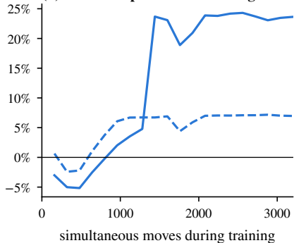
(b) HPWL improvement after legalization
