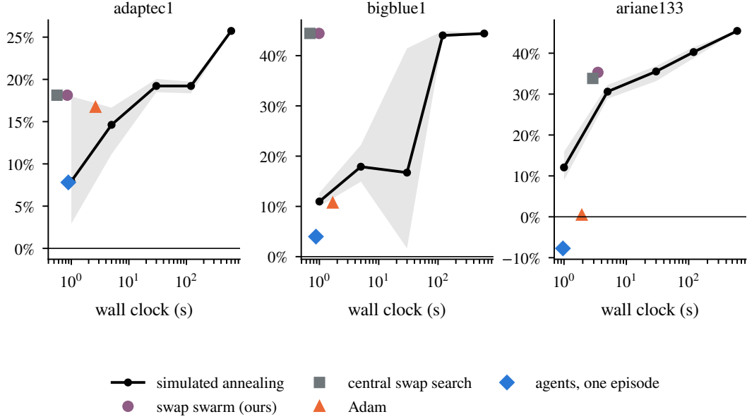
Figure 8: What each method reaches against the time it needs (log scale). The black line is simulated annealing at five budgets, with the band spanning its seeds. Markers are single runs of the other methods at their measured wall clock, including compilation.
