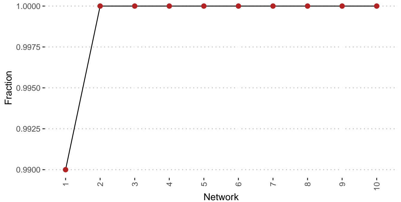
Giant component fraction
