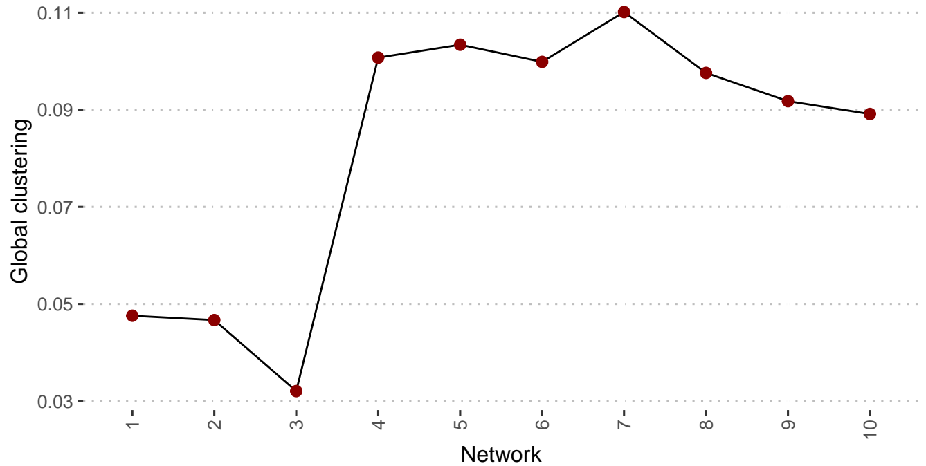
Global clustering
