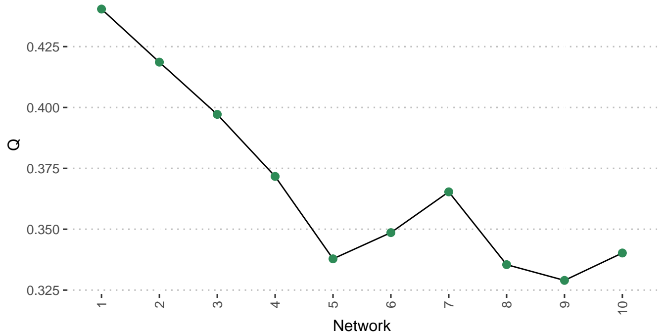
Q modularity
