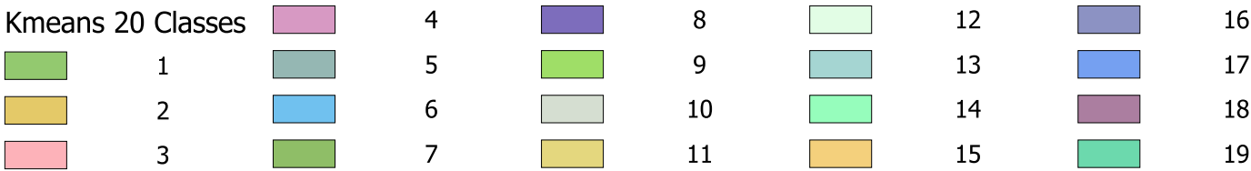
Spectral Classes
