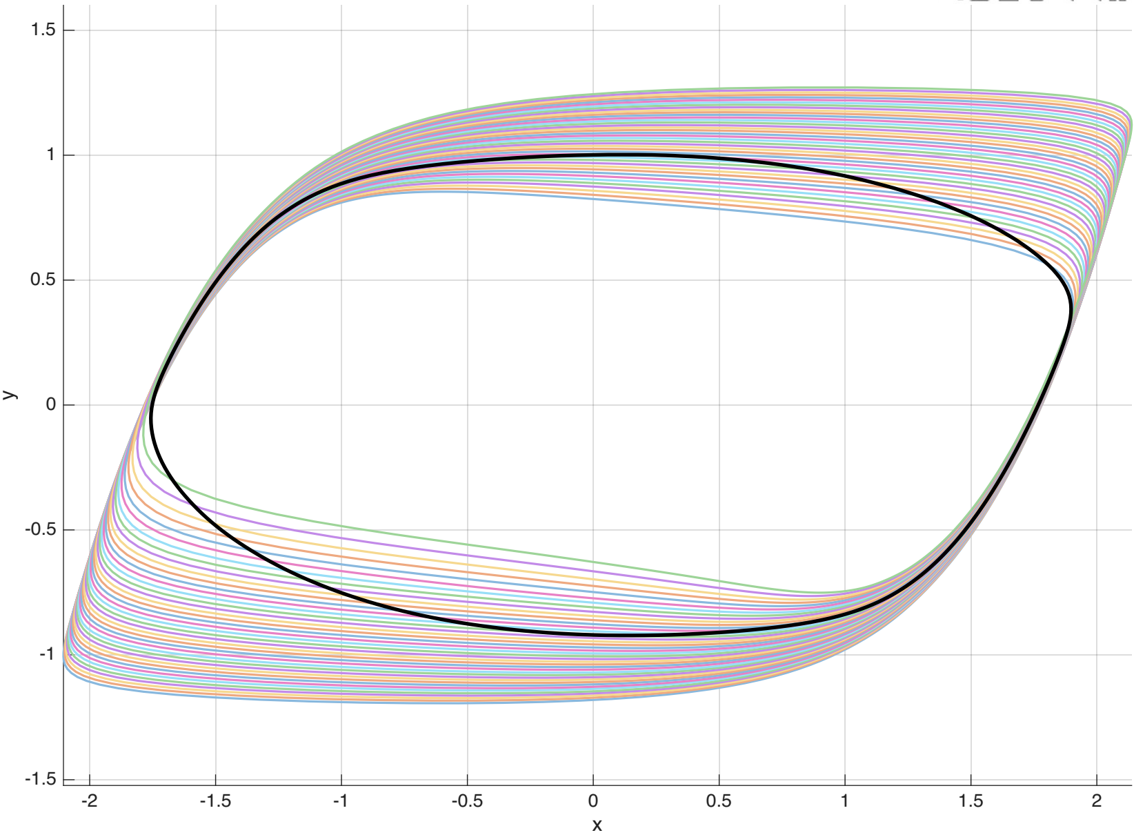
Fréchet mean
