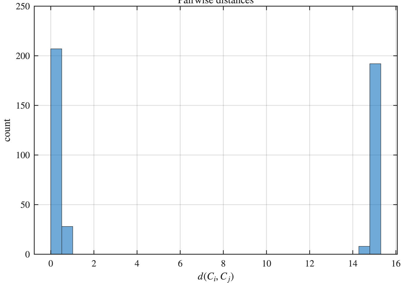
Pairwise distances
