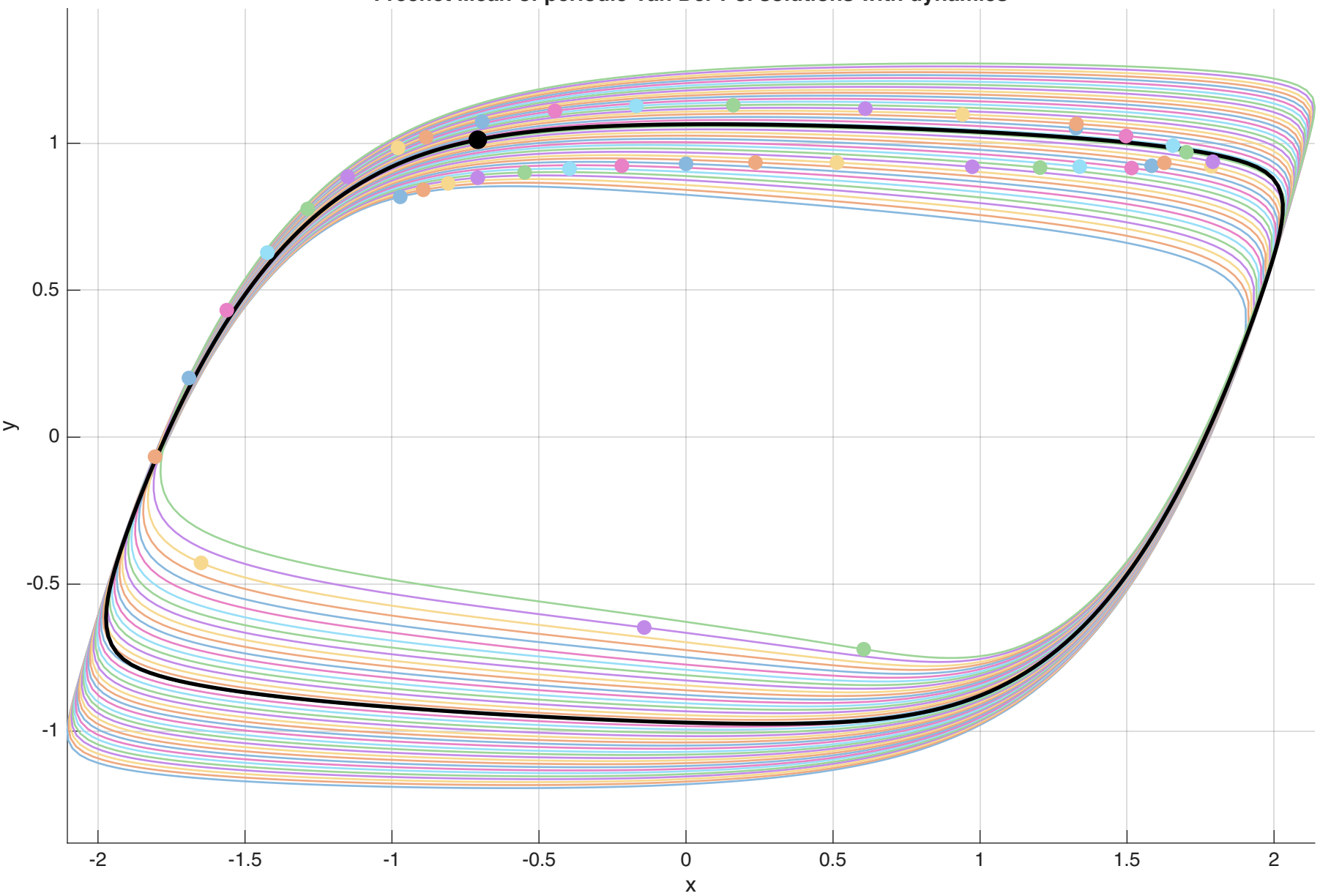
Fréchet Mean of periodic Van Der Pol solutions with dynamics
