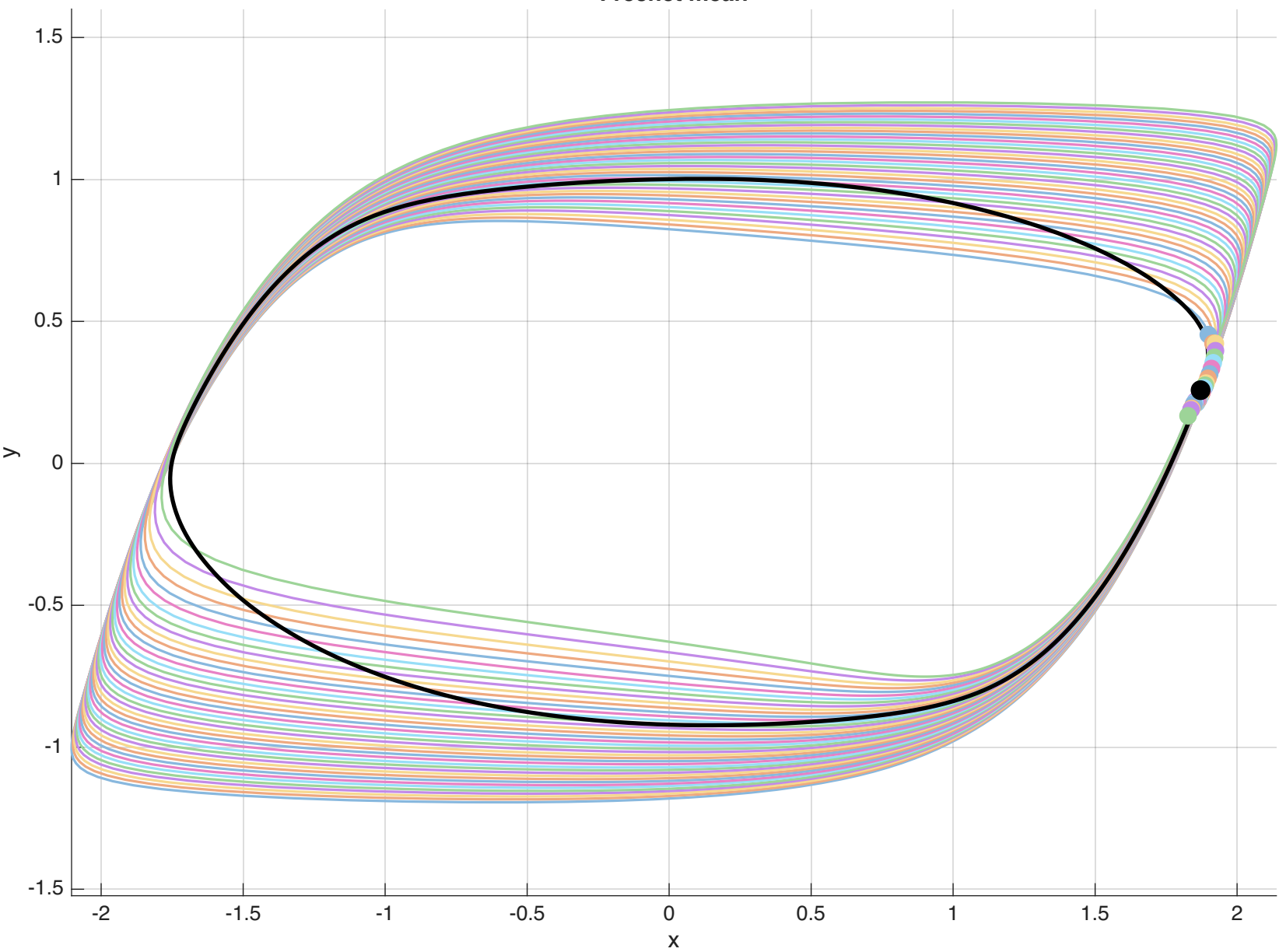
Fréchet mean
