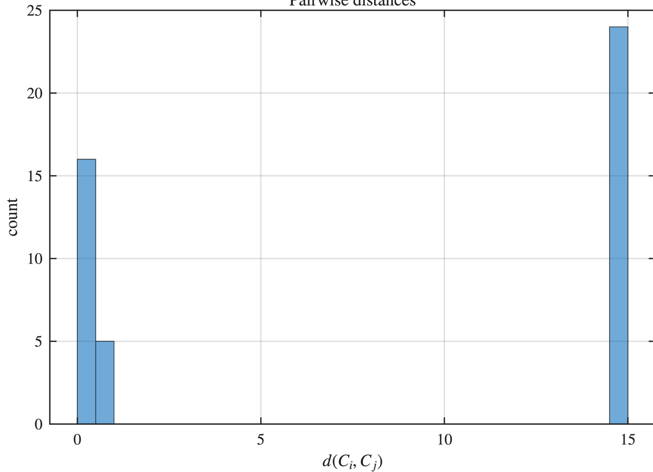
Pairwise distances
