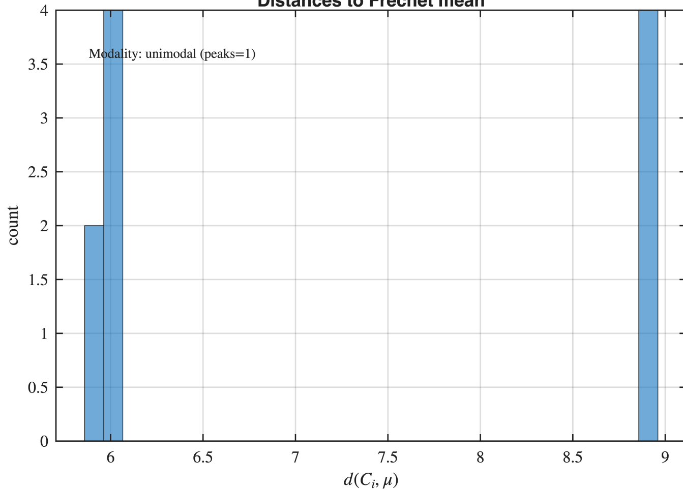
Distances to Fréchet mean
