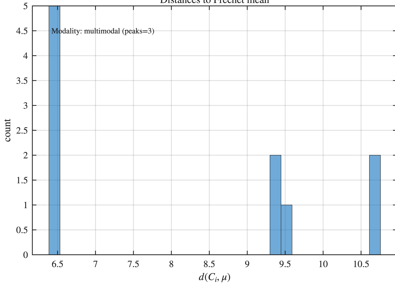
Distances to Frechet mean
