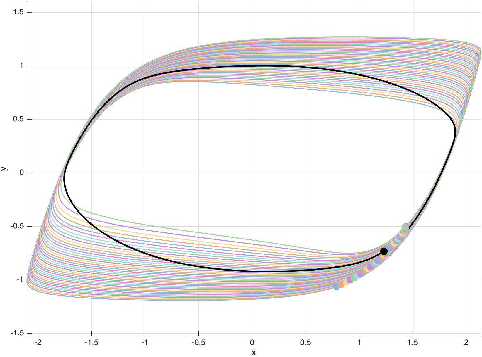
Fréchet mean
