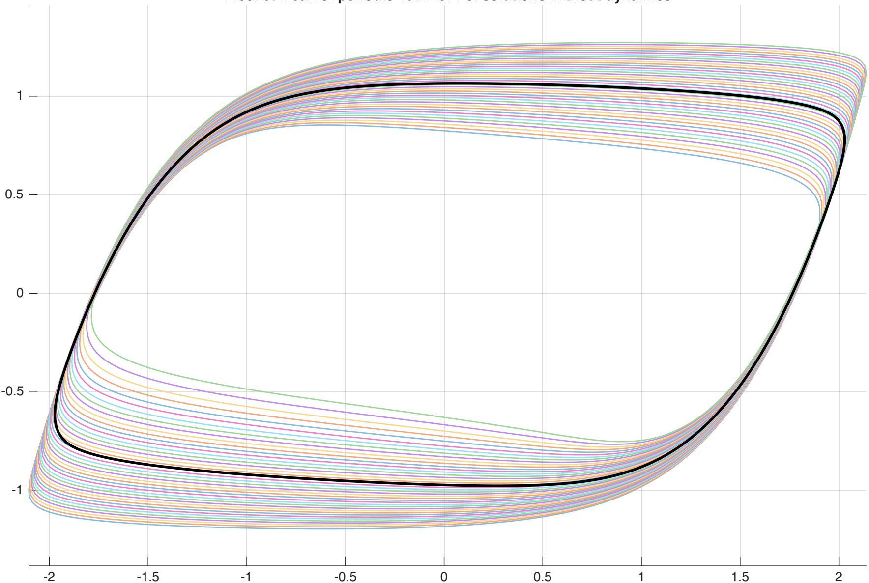
Fréchet Mean of periodic Van Der Pol solutions without dynamics
