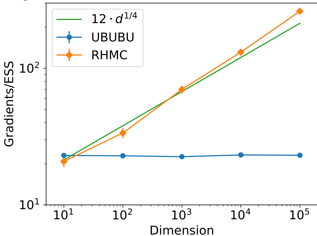
Max grads/ESS vs dimension - Coordinates - Gaussian \kappa = 100
