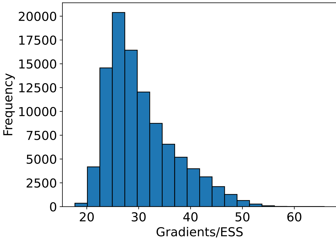
Gradients/ESS, coordinates, Gaussian \kappa = 4 , RHMC
