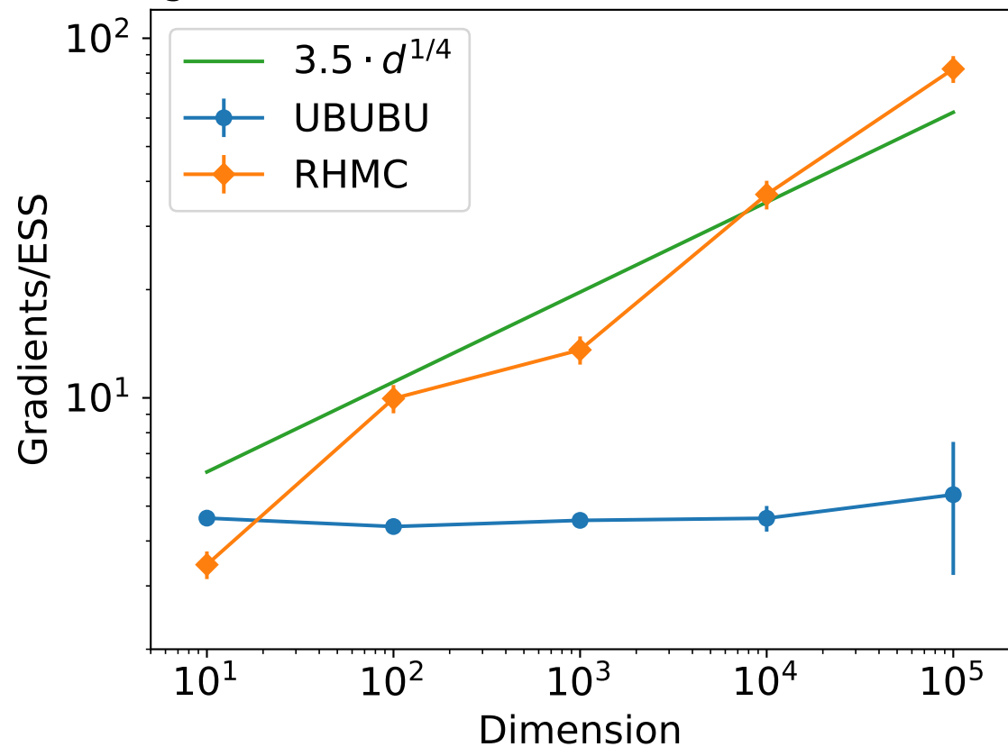
Max grads/ESS vs dimension - Norm - Gaussian \kappa = 4
