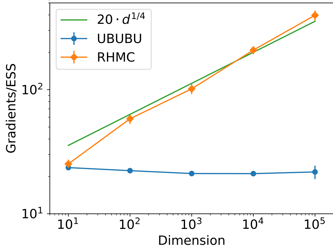
Max grads/ESS vs dimension - Norm - Gaussian \kappa = 100
