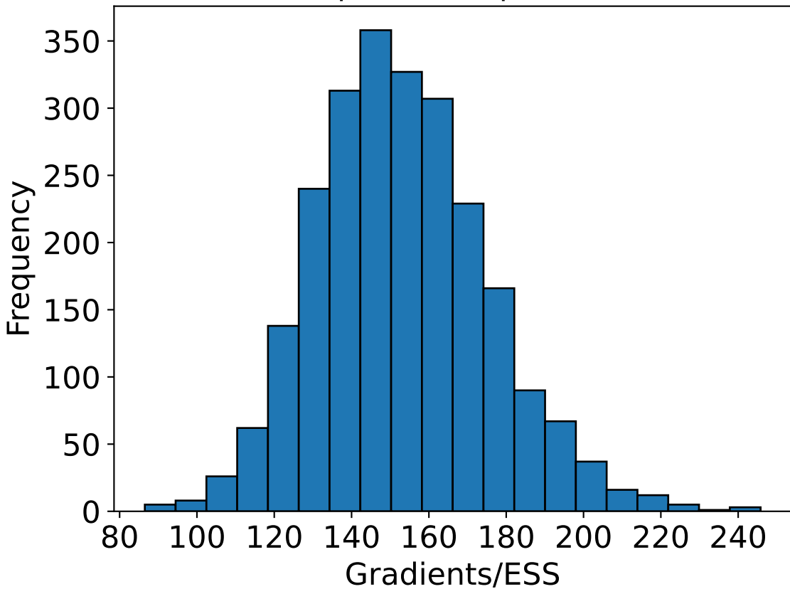
Gradients/ESS, prediction prob., MNIST, RHMC
