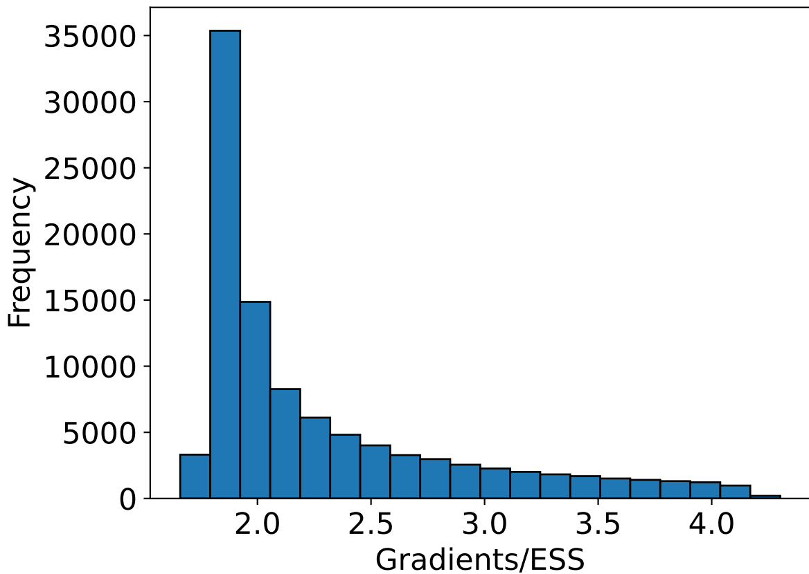
Gradients/ESS, coordinates, Gaussian \kappa = 4 , UBUBU
