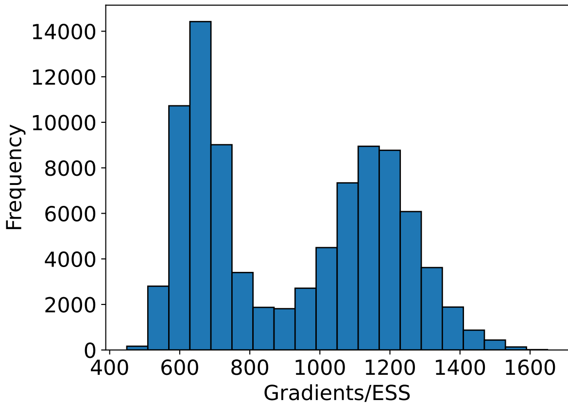
Grads/ESS, coordinates, Poisson model, RHMC
