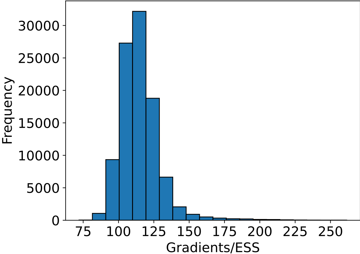
Histogram of Gradients/ESS, coordinates, Gaussian \kappa = 100 , RHMC
