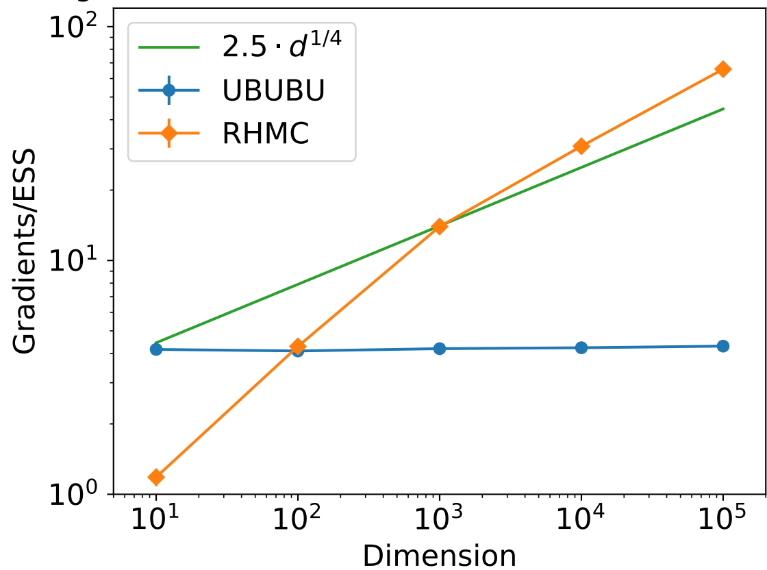
Max grads/ESS vs dimension - Coordinates - Gaussian \kappa = 4
