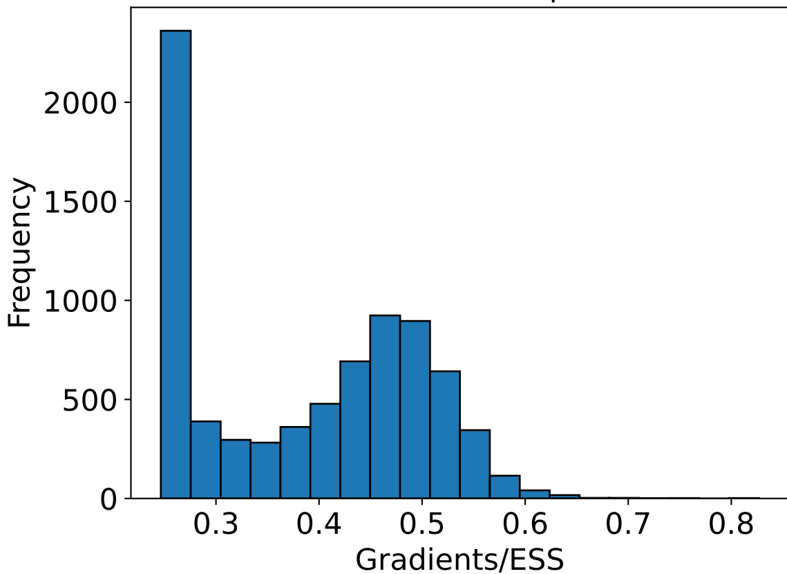
Grads/ESS, coordinates, MNIST, precondition. UBUBU-SG
