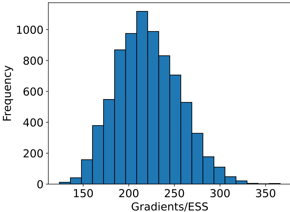
Gradients/ESS, coordinates, MNIST, RHMC
