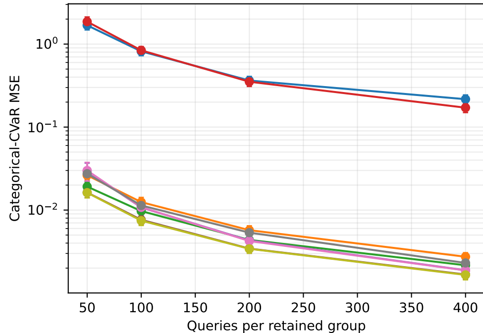
cliffwalking primary
