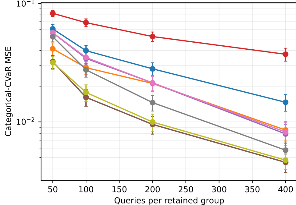
frozenlake 8x8
