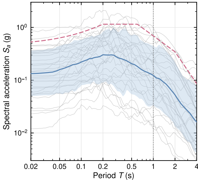
(a) 5%-damped acceleration response spectra
